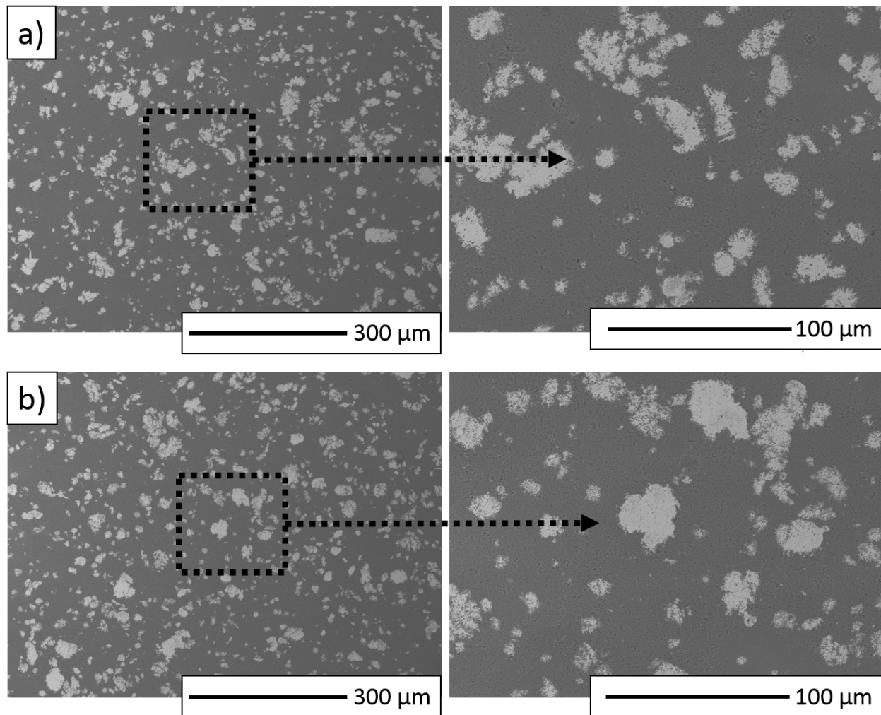
Fig. 2. SEM micrographs of cross-section of \text{Al}_2\text{O}_3 -Cu-Ni composite obtained by: (a) uniaxial powder pressing and (b) pulse plasma sintering
