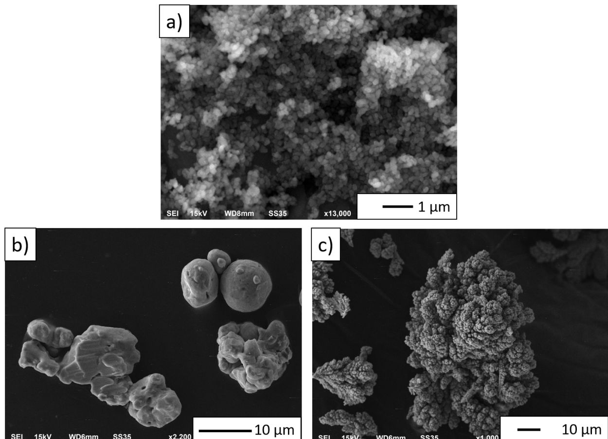
Fig. 1. Morphology of started powders: (a) alumina, (b) copper, (c) nickel powder
