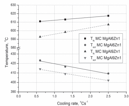
Fig. 10. Effect of cooling rate on nucleation ( T_N ) and solidus temperatures ( T_{sol} ) of investigated magnesium alloys
