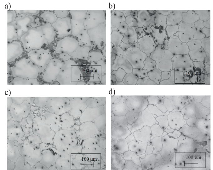
Fig. 8. Light microscope micrographs of the MC MgAl6Zn1: a-b) and MC MgAl9Zn1: c-d) alloys under 100x magnification that solidified at the following solidification rates: a, c) 0.6°Cs -1 ; b, d) 2.5°Cs -1
