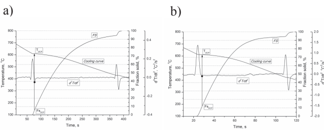
Fig. 11. Representative cooling and second derivative curves, and associated fraction solid curve of the MC MgAl6Zn1 alloy solidify at: a) 0.6°Cs -1 , b) 2.5°Cs -1 cooling rate
