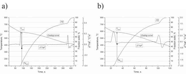
Fig. 12. Representative cooling and second derivative curves, and associated fraction solid curve of the MC MgAl9Zn1 alloy solidify at a) 0.6°Cs -1 , b) 2.5°Cs -1 cooling rate
