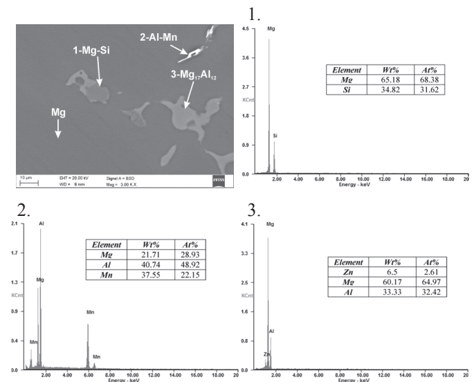
Fig. 4. Representative SEM micrographs of an MC MgAl6Zn1 alloy solidified at 0.6°Cs -1 cooling rate with EDS quantitative analysis results at marked points
