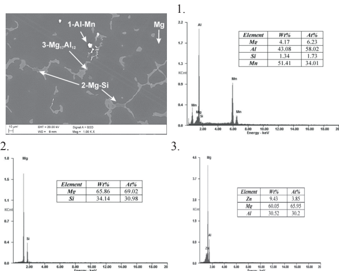
Fig. 6. Representative SEM micrographs of MC MgAl9Zn1 alloy solidify at 0.6°Cs -1 cooling rate with EDS quantitative analysis results at marked points
