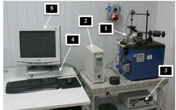
Fig. 3. Scheme of the T-11 position for the tribological pin-on-disc-type test: 1 - sensors and transducers, 2 - controller BT-11, 3 - controller BT-03, 4 - digital amplifier 8 Spider, 5 - a set of computers
