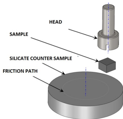
Fig. 5. Diagram of the steel and silicate counter-sample
