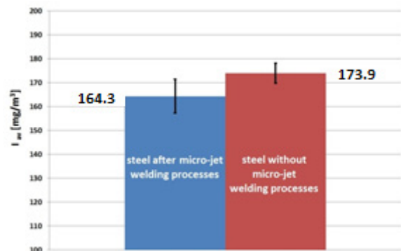
Fig. 6. Compilation of results for steel after padding with micro-jet cooling and without cooling
