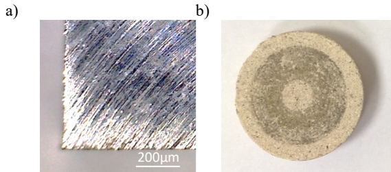
Fig. 4. View of: a) the sample, b) the counter-sample
