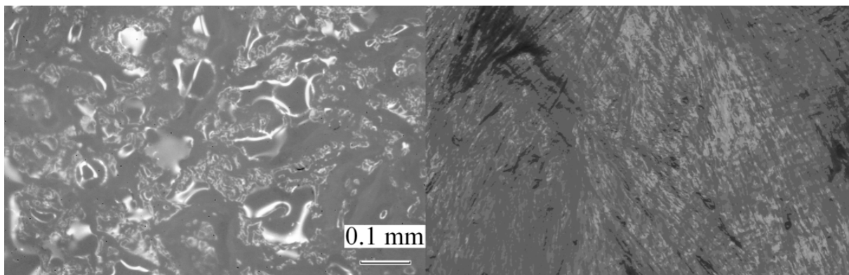
Fig. 2. AGO (left) and PVA-c (right) material microstructure, picture size of 600 x 900mkm; optical microscope (Nikon Microphot) image taken with a Nikon BD plan 5x/0.1 lens, pictures courtesy of Dr. W. Secomski.
