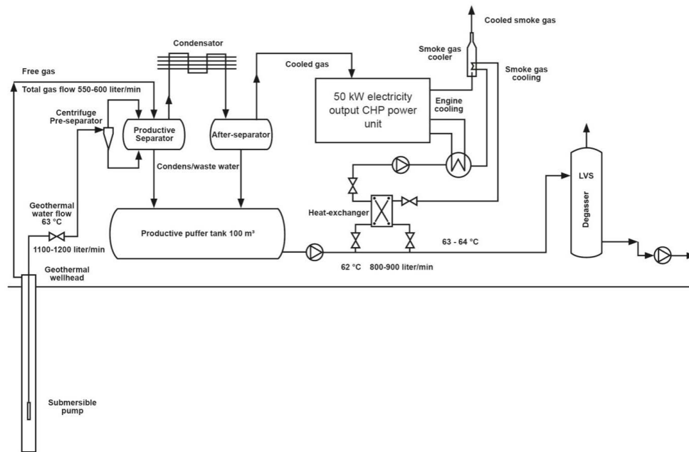
Fig. 1. Schematics of the waste gas utilization setup at the B-45 geothermal well site
