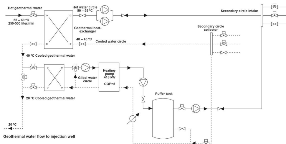
Fig. 2. Schematics of the heat-pump heating station
