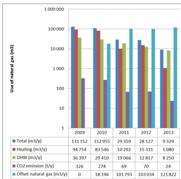
Fig. 6. Evolution of natural gas use at Morahalom
