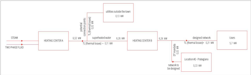
Fig. 3. Basic schematics of the district heating system of Montieri
