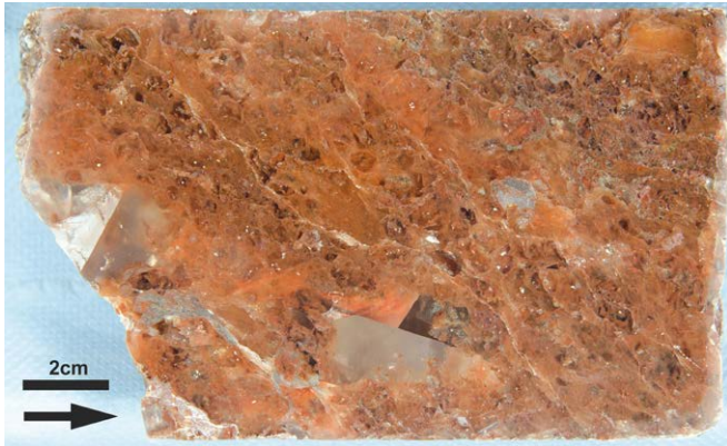
Fig. 10. Lower Tonbrockensalz (z4TSU): Polished surface of a core of the Go1004 (depth: 1808.30–1808.47 m); arrow points in drilling direction.
