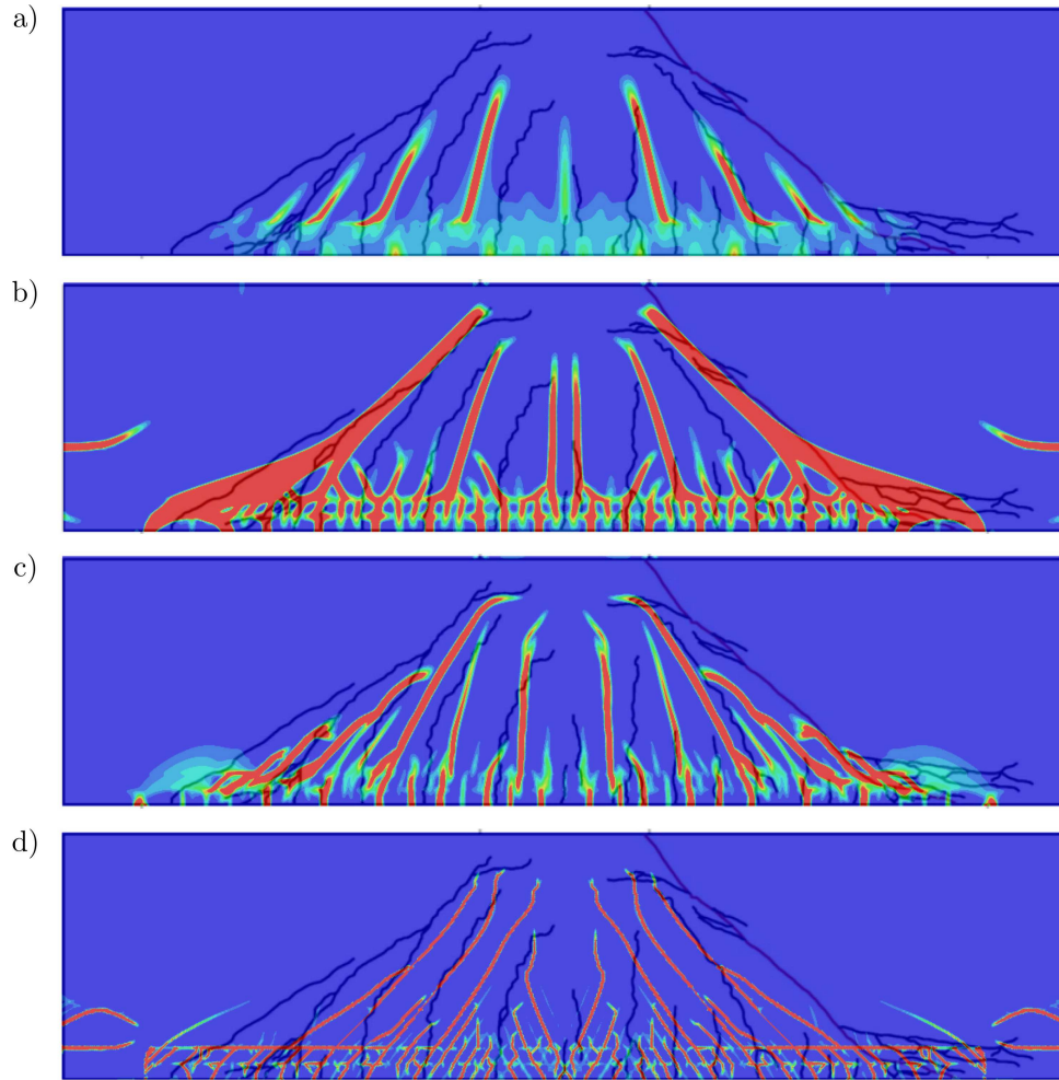
FIG. 9. Smearing crack patterns obtained with the: isotropic damage model (a), elasto-plastic model (b), coupled model (c) and concrete damaged plasticity model (d) for the beam S1D72a108.
