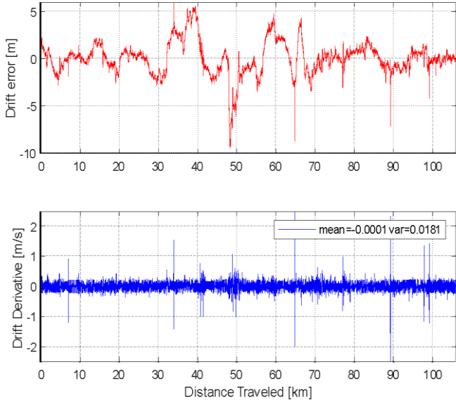
Fig. 17. Drift error (assuming temperature and pressure variability over time)
