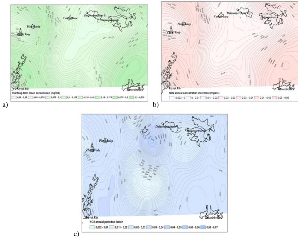
Fig. 3. Spatial distribution of time-series parameters of \text{NO}_2 content in atmosphere of Dnipropetrovs'k region for 2009–2014: a – average value of concentration ( \text{mg}/\text{m}^3 ), b – average annual increment of concentration ( \text{mg}/\text{m}^3 ), c – concentration annual periodic component
