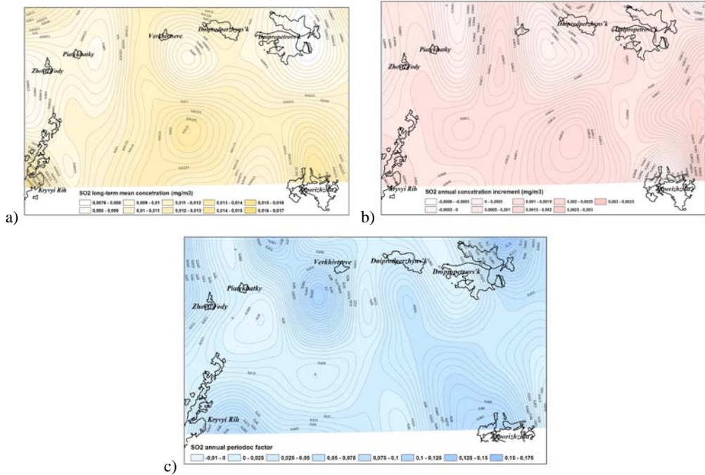
Fig. 4. Spatial distribution of time-series parameters of SO 2 content in the atmosphere of Dnipropetrovsk region for 2009 – 2014; a – average value of concentration (mg/m 3 ), b – average annual increment of concentration (mg/m 3 ), c – concentration annual periodic component
