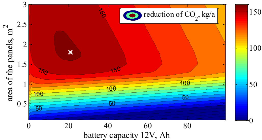
Fig. 3. Annually reduction of CO 2 emissions by PV systems as a function the battery capacity and the area of the panels Source: own study
