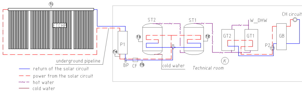
Fig. 2. Installation scheme: GT1 and GT2 – storage tanks supplied by gas boilers; GB – gas boiler; W_DHW – DHW outlet to the building; CH – the central heating circuit; P1 – solar circulation pump; P2 – boiler circulation pump; ST1 and ST2 – solar storage tanks, ETCHP – 15 tube evacuated tube collectors; BP – by-pass; CF – heat meter; T1...5 – temperature sensors; CW – cold water inlet Source: own study
