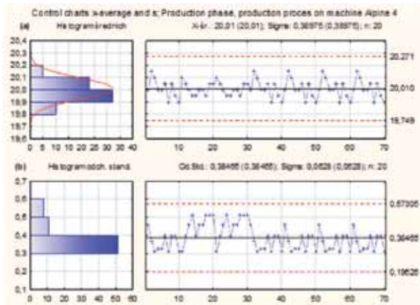
Fig. 6. (a) The average of the mean values of thickness measurements from the Alpine 4 machine; (b) average standard deviations of thickness measurements from the Alpine 4 machine
