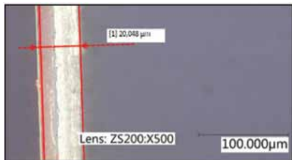
Fig. 3. A microscopically magnified cross section of the PE film and the results of the measurement
