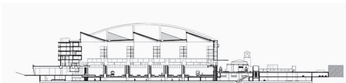
Fig. 15. Zaragoza Delicias, section source: Ferrater, C. (2011). OAB Carlos Ferrater and Partners. N.p.: Actar.
