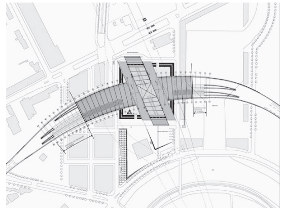
Fig. 19. Berlin Hauptbahnhof, source: http://www.constructalia.com/repository/transfer/en/resources/ContenidoProject/01666451Foto_big.jpg
