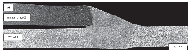
Fig. 2. Macrostructure of the overlap joints of Grade 2 titanium – aluminium alloy AW-5754 braze welded with Al99.5 filler metal \varnothing 2.4 mm, titanium on the top (a) titanium at the bottom (b), chemical etching using Kroll's reagent
