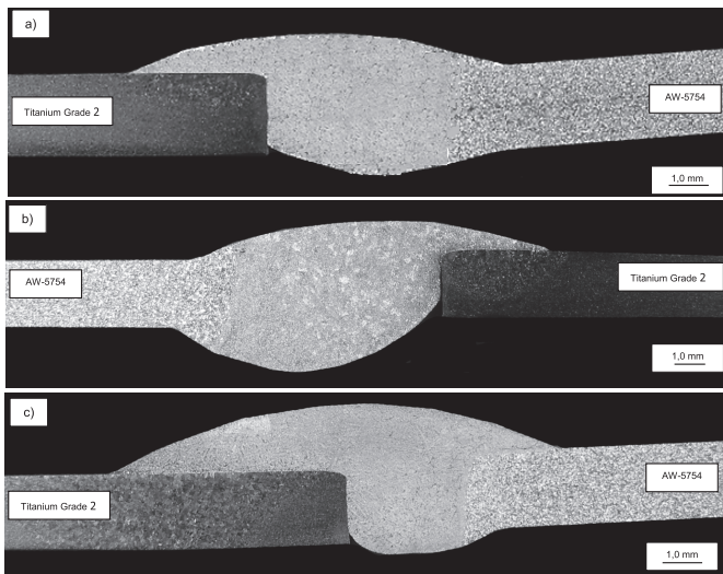
Fig. 1. Macrostructure of the butt joints of Grade 2 titanium – aluminium alloy AW-5754 braze welded with filler metals Al99.5 (a), AlSi5 (b), AlSi12 (c), chemical etching using Kroll's reagent
