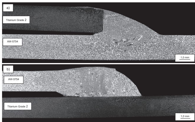
Fig. 2. Macrostructure of the overlap joints of Grade 2 titanium – aluminium alloy AW-5754 braze welded with Al99.5 filler metal \varnothing 2.4 mm, titanium on the top (a) titanium at the bottom (b), chemical etching using Kroll's reagent
