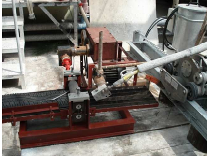
Fig. 8. Tests on flat tyre
