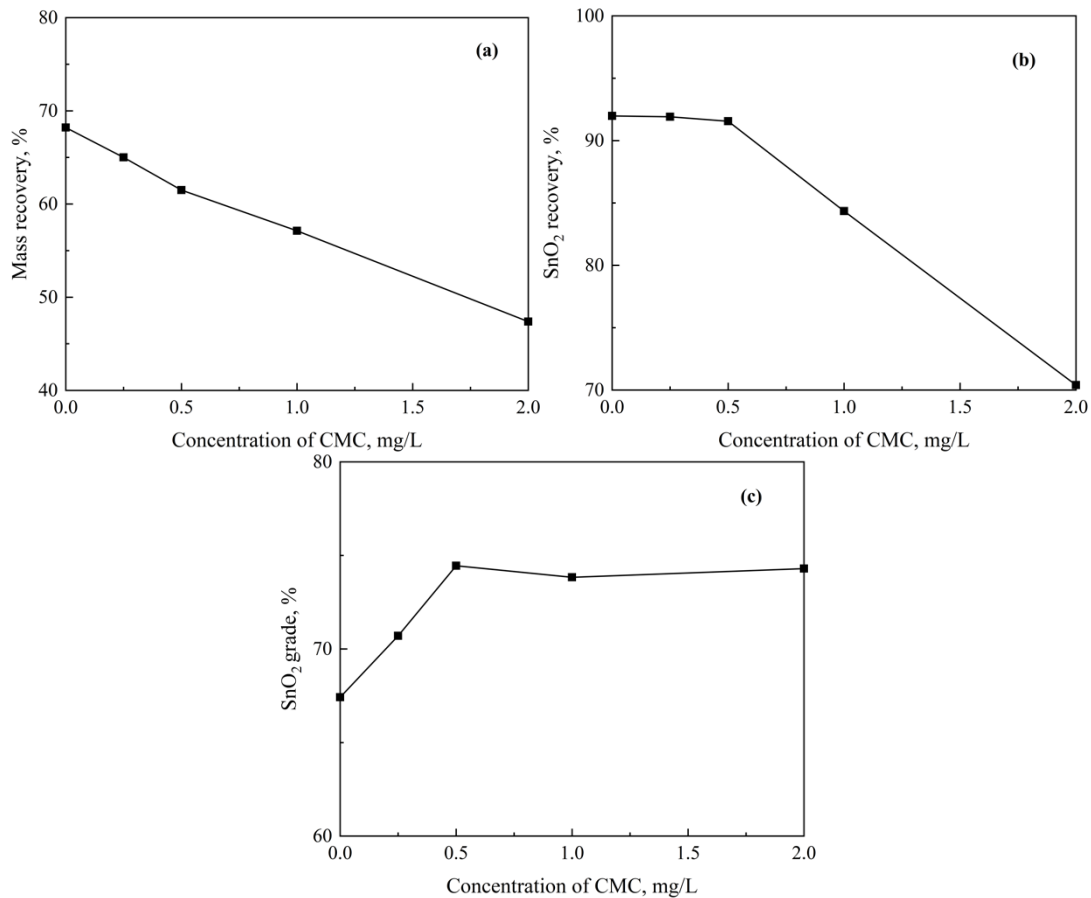
Fig. 8. (a) The mass recovery; (b) \text{SnO}_2 recovery; and (c) \text{SnO}_2 grade of flotation concentrates as a function of CMC concentration ( c(\text{BHA})=60 \text{ mg/L} , c(\text{LN})=30 \text{ mg/L} , c(\text{MIBC})=10 \text{ mg/L} )
