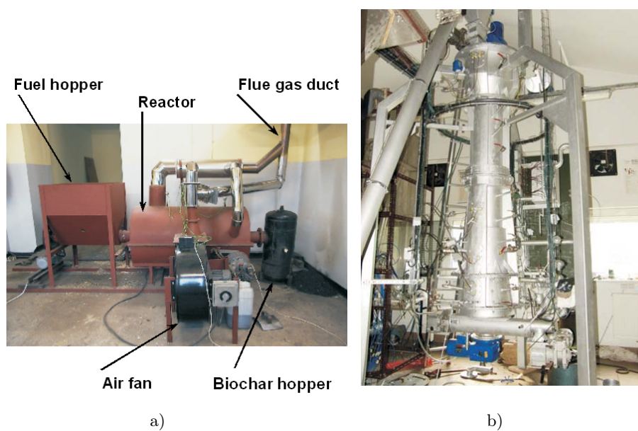
Figure 1. Examples of horizontal (a) and vertical (b) reactors for the thermal treatment of biomass fuels at the Czestochowa University of Technology.
