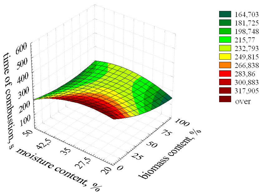
Fig. 6. The influence of suspension moistness and biomass content in suspension on the fuel combustion time in a fluidized bed; T = 850^{\circ}\text{C}
