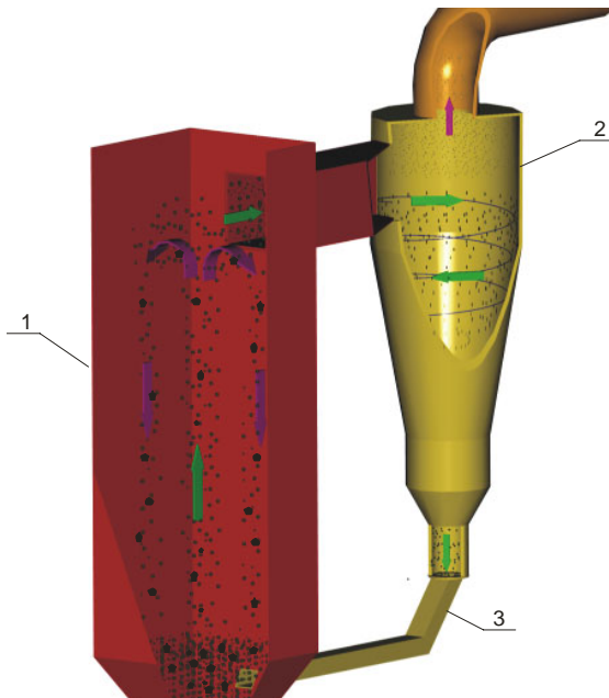
Fig. 1. Average movement of fuel particles in the boiler with a circulating fluidized bed 1 – combustion chamber, 2 – cyclone, 3 – system of material return — internal circulation; — contour circulation
