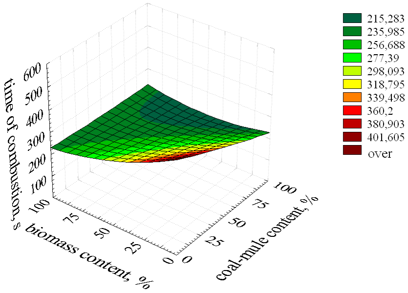
Fig. 7. The influence biomass and coal-mule content in suspension on the fuel combustion time in a fluidized bed; T = 850°C
