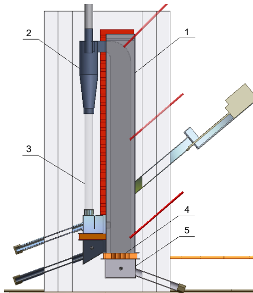
Fig. 3. The section of the research stand for fuel combustion in a stream of air and in a circulating fluidized bed and the process visualization; 1 – fluidized column, 2 – cyclone, 3 – return system, 4 – no-pouring fire grate, 5 – air box
