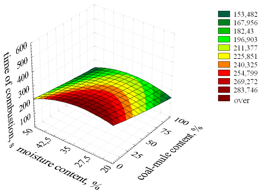
Fig. 9. The influence of suspension moistness and coal-mule content in suspension on the fuel combustion time in a fluidized bed; T = 850^{\circ}\text{C}
