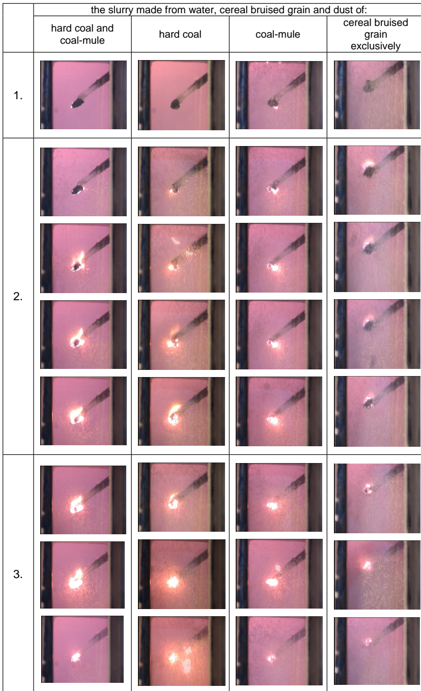
Fig. 11. Example of a course of coal-water fuel combustion process in the fluidized bed; 1 – heating and vaporization of moisture, 2 – devolatilization, ignition and combustion of volatiles matter, 3 – combustion of char-suspension; W = 35\% ; T = 850^{\circ}\text{C} (Kijo-Kleczkowska, 2008-2010)
