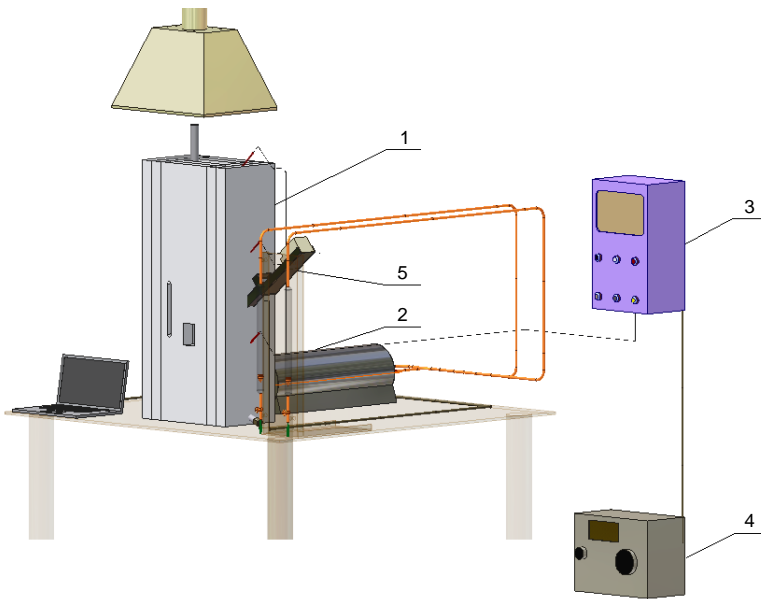
Fig. 2. The research stand for fuel combustion in a stream of air and in a circulating fluidized bed and the process visualization; 1 – fluidized column, 2 – gas heater, 3 – control box, 4 – power driver, 5 – fuel introduction system
