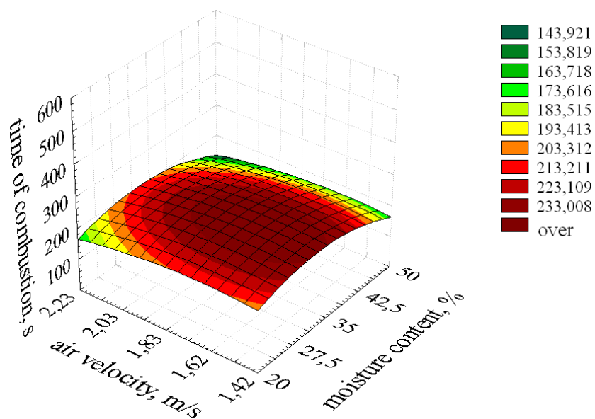
Fig. 10. The influence of suspension moistness and air flow velocity on the fuel combustion time in a fluidized bed; T = 850^{\circ}\text{C}
