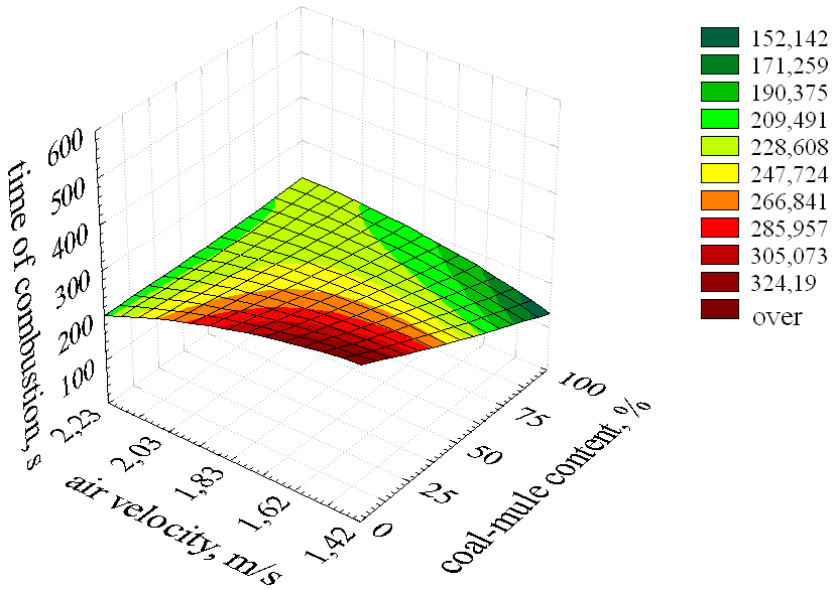
Fig. 8. The influence of air flow velocity and coal-mule content of suspension on the fuel combustion time in a fluidized bed; T = 850°C
