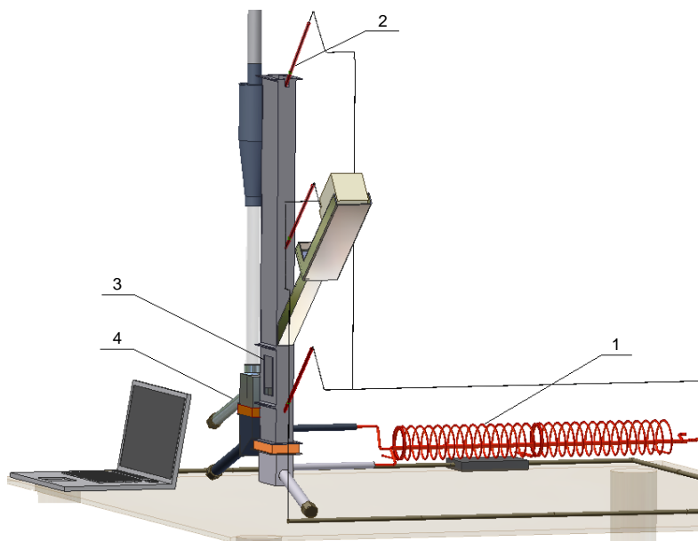
Fig. 4. The research stand for fuel combustion in a stream of air and in a circulating fluidized bed (without insulation) ; 1 – gas heater, 2 – thermocouple Ni-CrNi, 3 – visualization pane, 4 – inert material pouring out place of fluidized bed material
