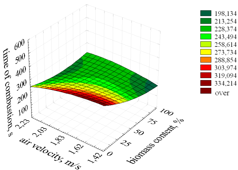
Fig. 5. The influence of air flow velocity and the biomass content in suspension on the fuel combustion time in a fluidized bed; T = 850^{\circ}\text{C}
