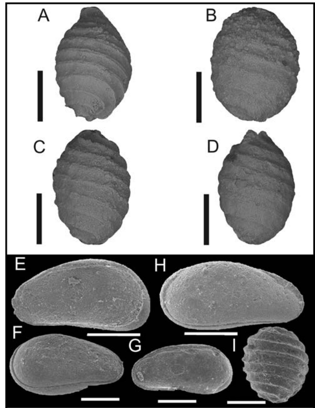
Fig. 17. Typical association of charophyte algae (A–D, I) and ostracods (E–G) from the Norian Grabowa Fm (Olempska et al. , 2012). A. Stellatochara . B, I. Porochara . C. Stenochara . D. Stomochara . E, F, G. Suchonella sp. H. Darwinula oblonga (Römer). Woźniki K1 well, depth 30.5 m (A–D), Patoka 1 well, depth 176.1 m (E–G); Woźniki K1 well, depth 18.5 m (I). Scale 200 \mu m.
