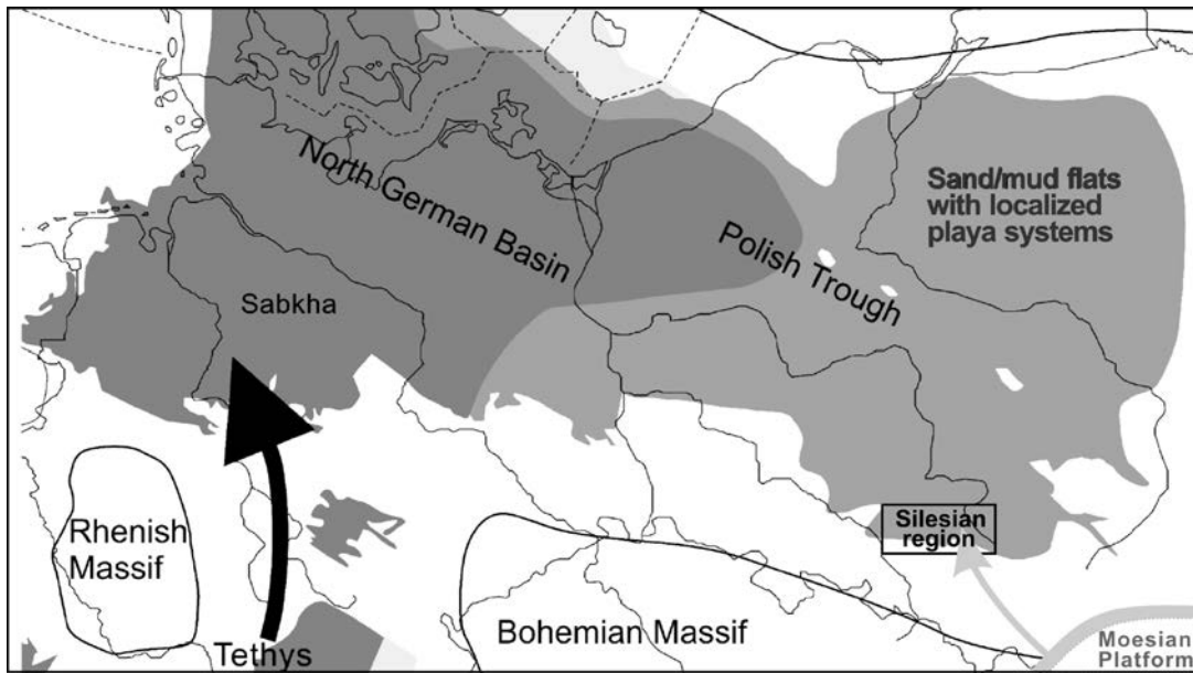
Fig. 4. Palaeogeographic location of Upper Silesia region and present-day distribution and facies map of the Norian (Steinmergelkeuper, modified from Feist-Burkhardt et al. , 2008, fig. 13.24B). Solid lines represent the reconstructed eastern Germanic Basin outline, the black arrow indicates the marine ingression from the Tethys Ocean and the grey ones illustrate possible clastic supply from the Moesian terrane (see Fig. 5).
