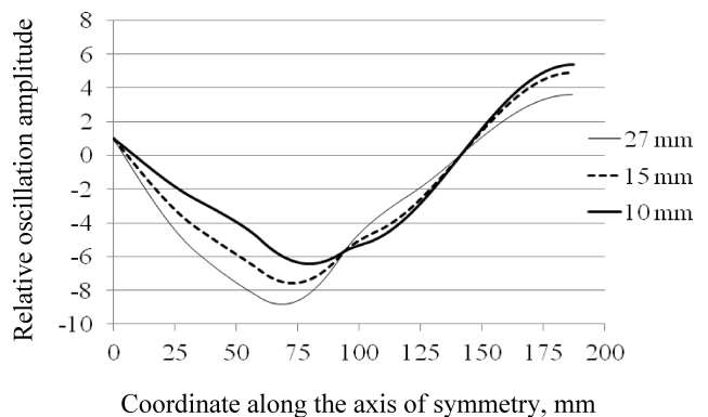
Fig. 3. Distribution of the amplitudes of longitudinal vibrations of concentrating link at different lengths of the zone l_4 .
