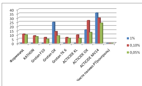
Pic.1. Comparative distribution of research results of fuels biological stability, protected by biocide additives by diffusion zone method
