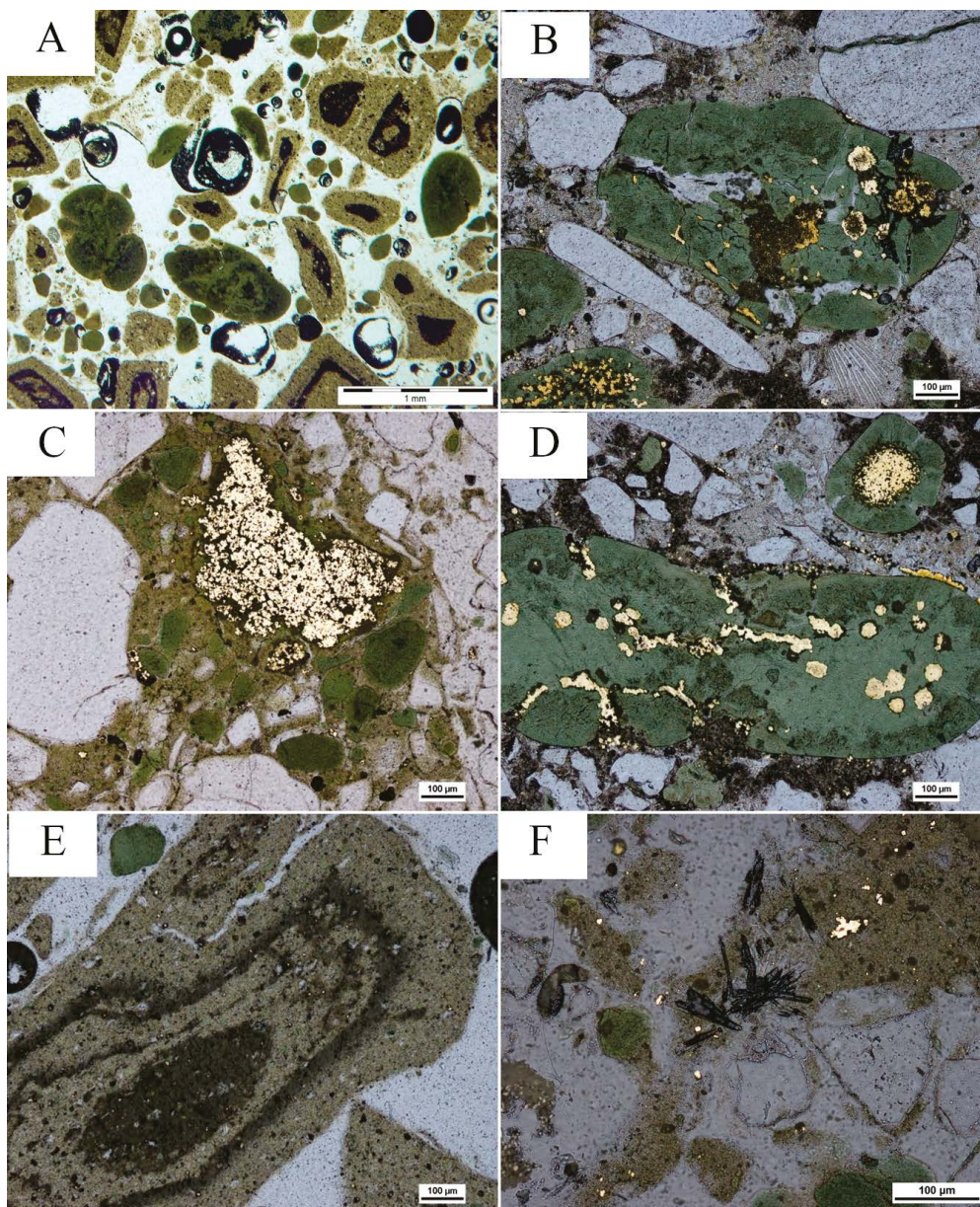
Fig. 3. Photomicrographs of quartz-glaucinite sand from the “Górka Lubartowska-Nieźwiada” deposit (NX/IN). A – poor degree of sorting and a medium degree of roundness of the analytical material; B, C, D – euhedral and/or framboidal forms of pyrite aggregations within glauconite grains; E – clay aggregates; F – rosette gypsum crystals
