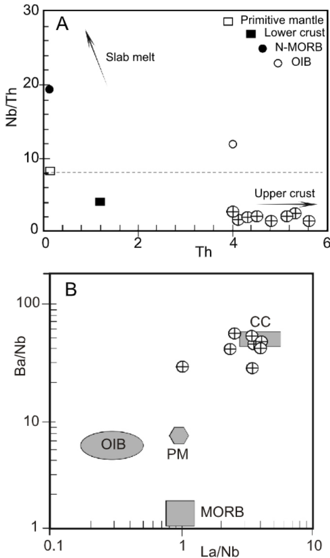
Fig. 9A – plot of Nb/Th vs. Th for the mafic dykes; B – plot of Ba/Nb vs. La/Nb for the rocks
