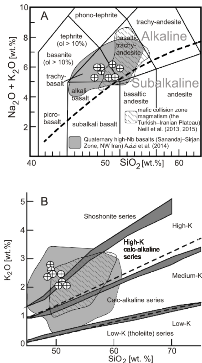
Fig. 5A – Na 2 O + K 2 O vs. SiO 2 discrimination diagram with field delineated after Middlemost (1994); B – K 2 O vs. SiO 2 discrimination diagram (Rickwood, 1989)
