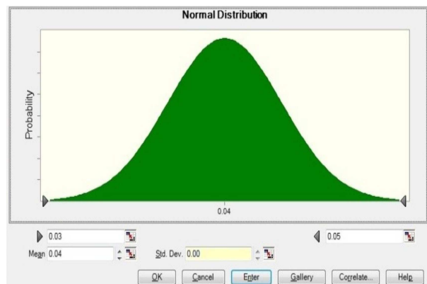
Fig. 5. Normal distribution of inflation rate – 2002 with mean and standard deviation.
