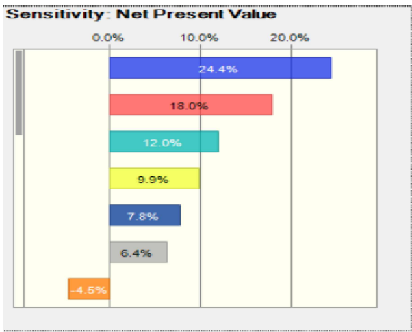
Fig. 9. Sensitivity analysis chart of net present value.
