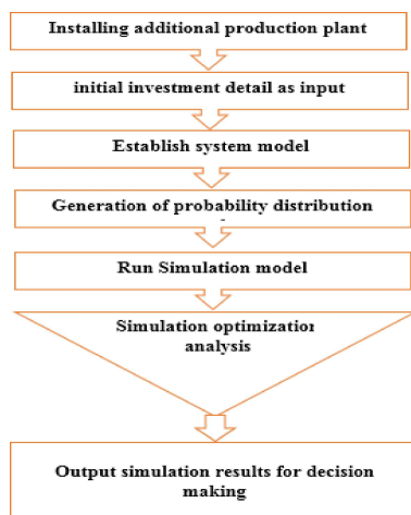
Fig. 2. General steps flow chart of simulation.
