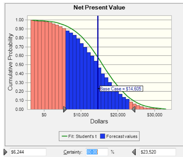
Fig. 11. Net present value reverse cumulative frequency distribution.
