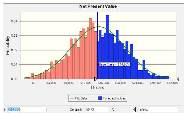
Fig. 7. Net present value certainty results with $14,606.
