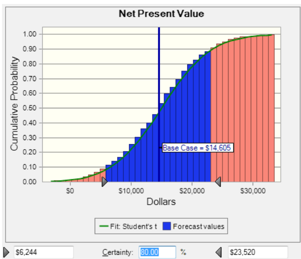
Fig. 10. Net present value cumulative frequency distribution.
