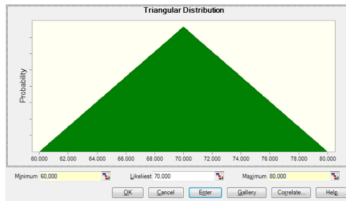
Fig. 4. Triangular probability distribution.
