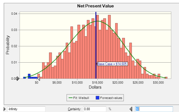
Fig. 8. Net present value certainty results with $0.00.
