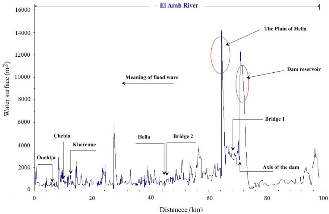
Fig. 13. The surface of the water during the flood; source: own study
