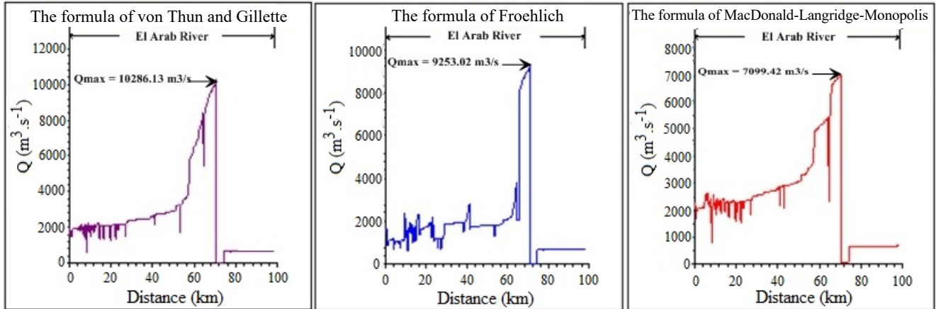
Fig. 7. The evolution of the flood wave by the three empirical methods; source: own study
