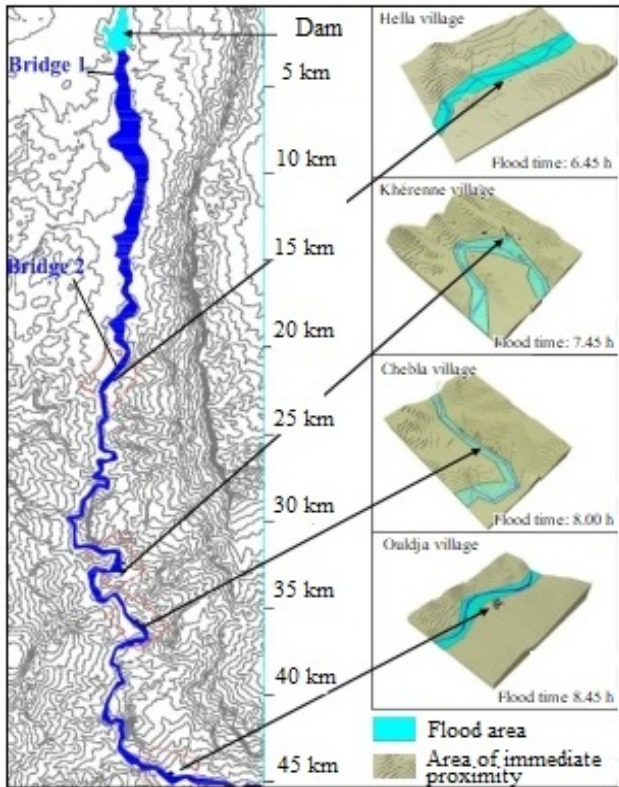
Fig. 16. Map of flooding by dam failure Babar; source: own study
