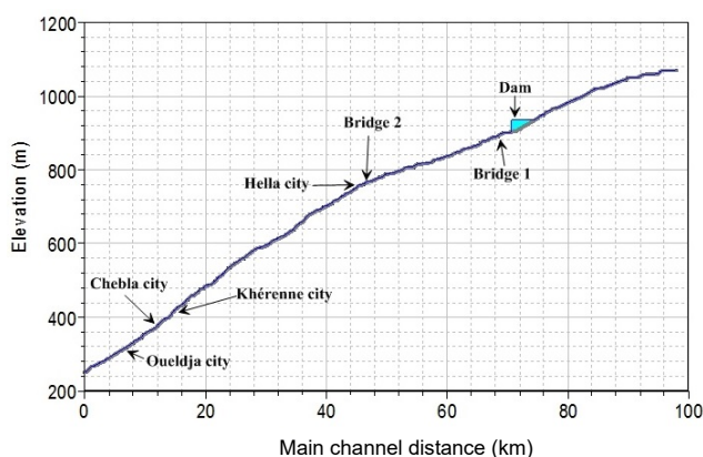
Fig. 2. Longitudinal profile of the El Arab River section near the dam; source: own elaboration
