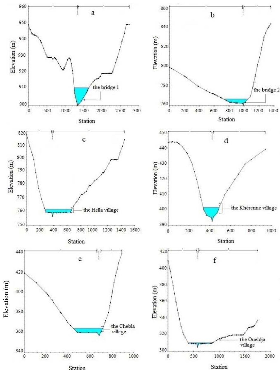
Fig. 15. The water level after the failure at: a) the bridge 1, b) the bridge 2, c) the Hella village, d) the Khérenne village, e) the Chebla village, f) the Oueldja village; source: own study
