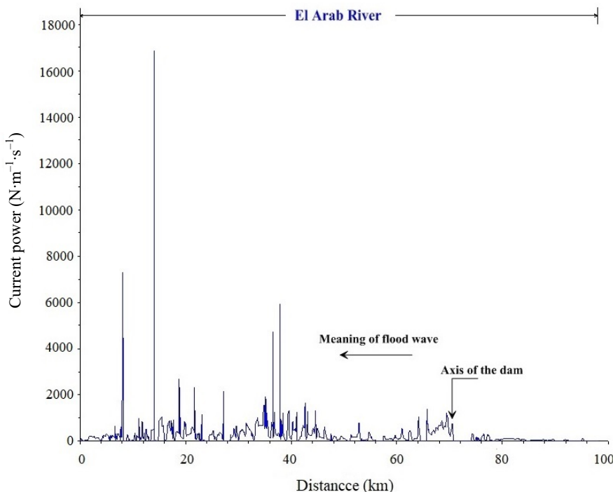
Fig. 12. Water current power of the flood wave; source: own study
