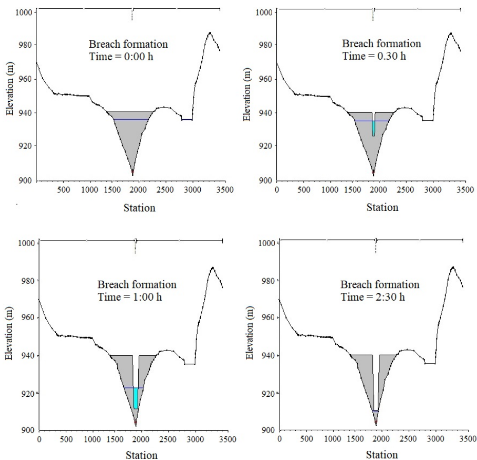
Fig. 8. Dam failure and formation breach in time; source: own study
