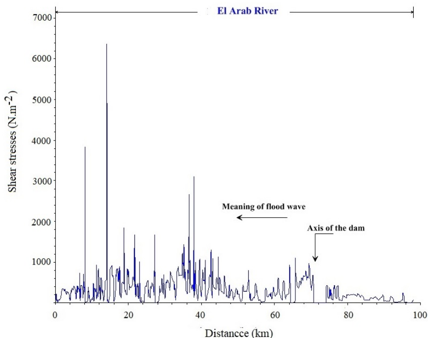
Fig. 11. Shear stress and the transport of the bed of the El Arab River; source: own study
