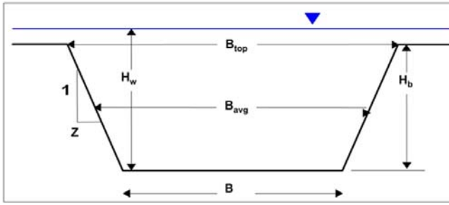
Fig. 6. Breach profile type; source: own elaboration
