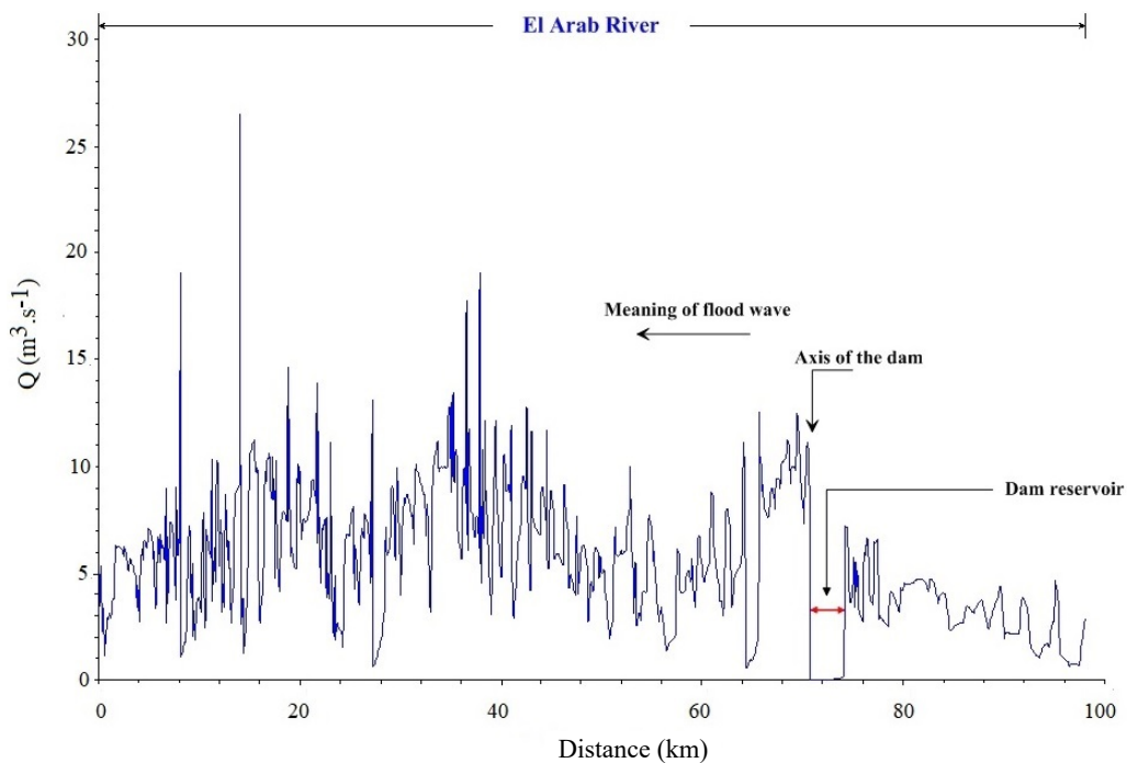
Fig. 10. Variation in flood wave velocity after dam failure; source: own study
