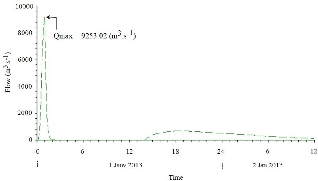
Fig. 14. Breach hydrographs at dam; source: own study
