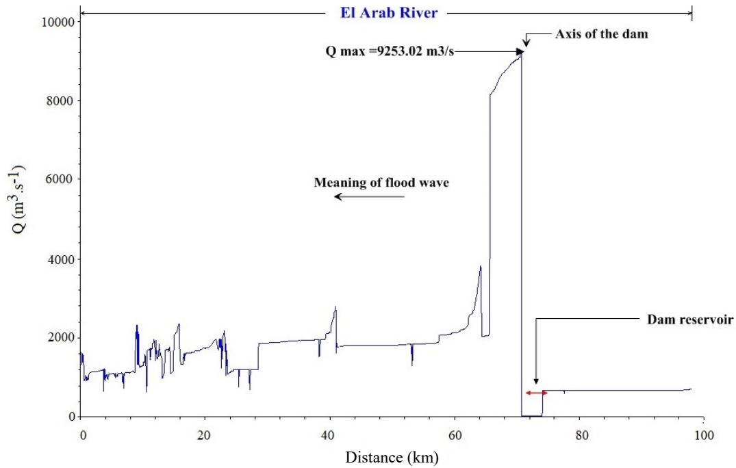
Fig. 9. Variation in flowrate after dam's failure; source: own study
