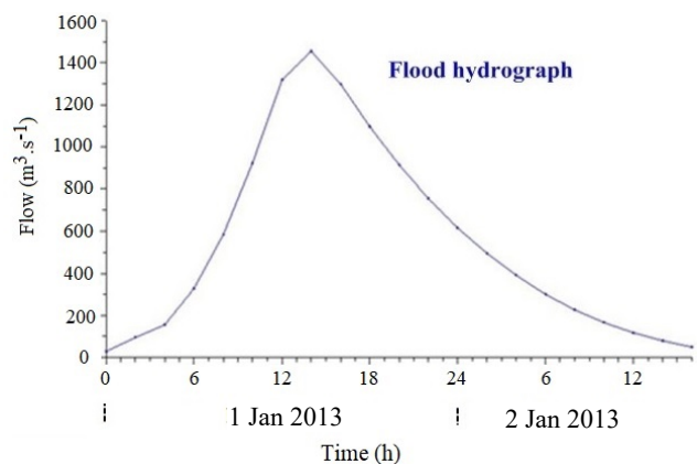
Fig. 5. Dam inlet flood hydrograph; source: own elaboration
