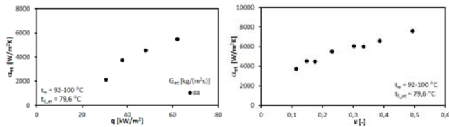
Fig. 20. Heat transfer coefficient on heat exchanger ethanol side vs. heat flux.
