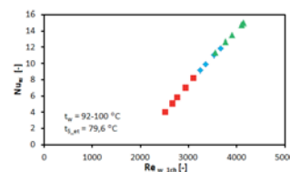
Fig. 18. Nusselt number vs. water flow Reynolds number for one minichannel.
