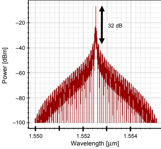
Fig. 3. Simulation optical spectra of the generated optical mm-wave with DD-MZM2 based at the maximum transmission point.
