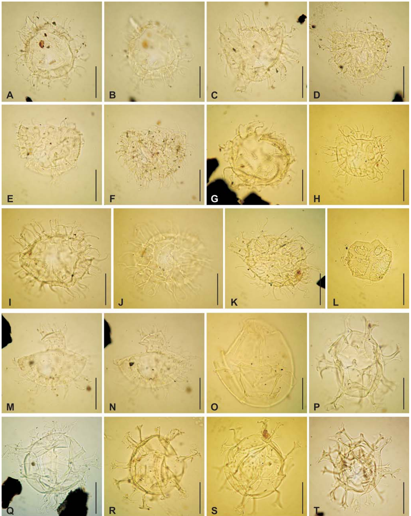
Fig. 7. Dinoflagellate cysts from upper Badenian at Józefów. Scale bars = 25 µm. A–L. Cleistosphaeridium placacanthum (A–F, I, J: Pds-2; A, B – same specimen, various foci; G, H, K, L: Pds-1; L – isolated operculum). M, N. Lingulodinium machaerophorum (same specimen with 5P archaeopyle, various foci; Pds-2); O. Pentadinium sp. (Pds-1). P–T. Spiniferites pseudofurcatus (P, Q: Pds-2; R–T: Pds-1).
