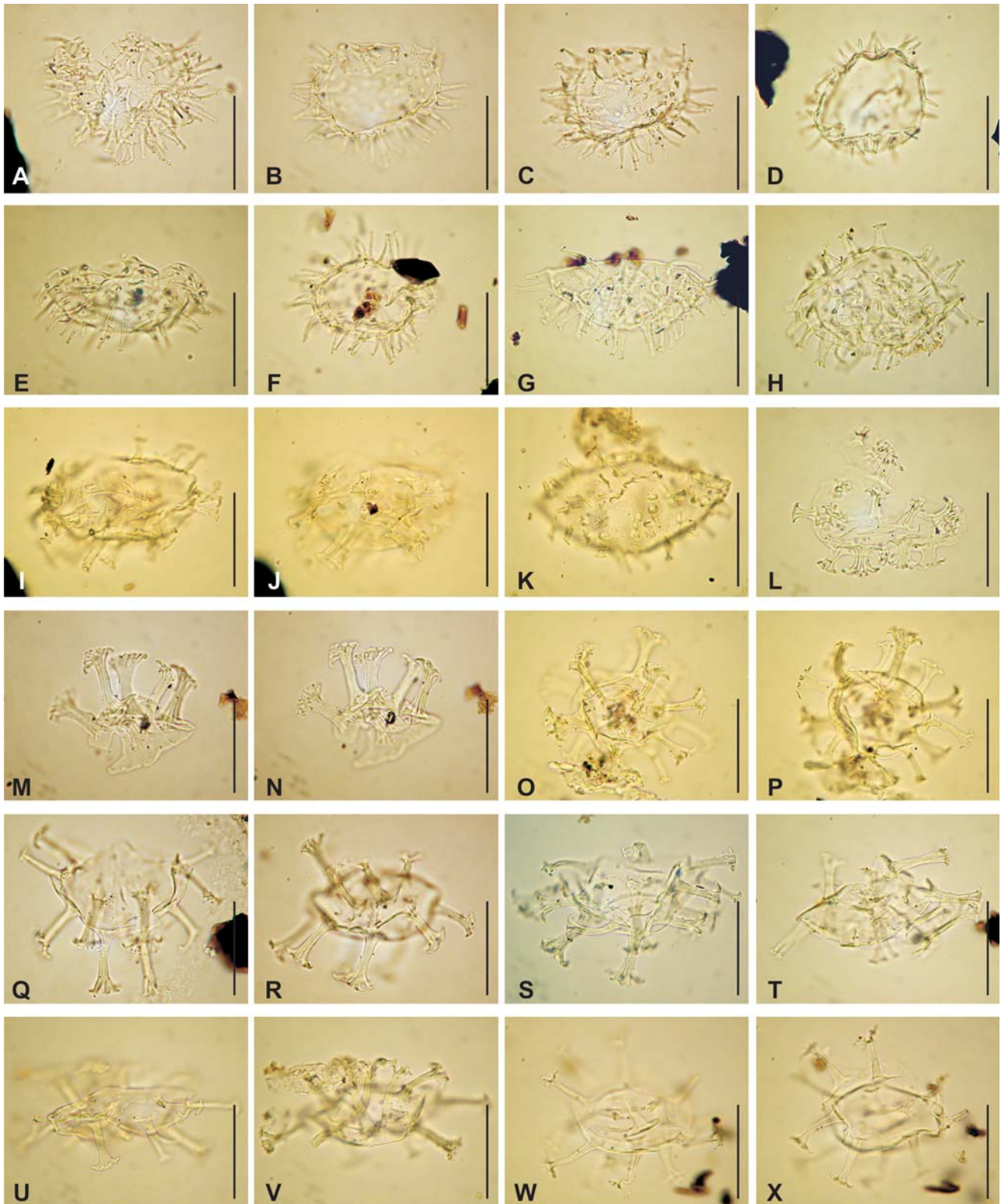
Fig. 8. Dinoflagellate cysts from upper Badenian at Józefów. Scale bars = 25 \mu m. A–F. Polysphaeridium subtile (A–E: Pds-1; F: Pds-2; B, C: same specimen, various foci); G–K. Polysphaeridium zoharyi (all specimens: Pds-1; J, K: same specimen, various foci); L. Homotryblium vallum (presumably reworked; Pds-1); M–S. Homotryblium floripes (M–R: Pds-1; S: Pds-2; M, N and O, P: same specimens, various foci); T–V. Homotryblium plectilum (all specimens: Pds-2); W, X. Homotryblium tenuispinosum (Pds-2; same specimen, various foci).
