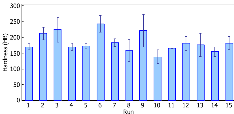
Fig. 1. Variations of hardness values of the cast iron samples produced in various compositions
