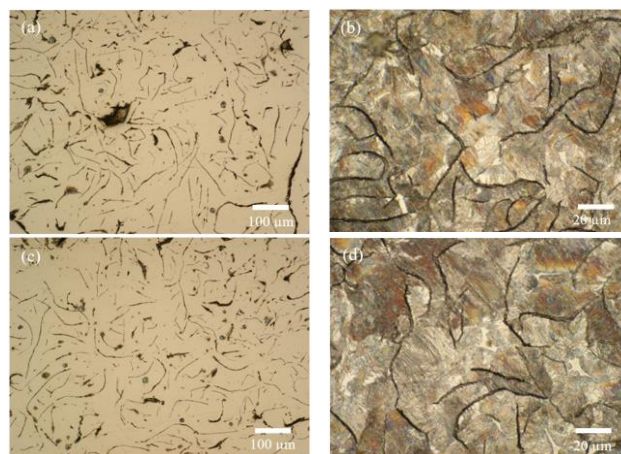
Fig. 5. Stereomicroscopy images of microstructures of cast irons obtained (a) and (b) from the company (c) and (d) from this study
