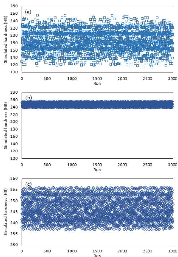
Fig. 4. Variations of simulated hardness values after performing MCS on different proportions of components for (a) previous constraints (b) and (c) for appropriate proportion of the four components
