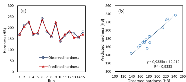
Fig. 2. Actual observations and predicted values of hardness
