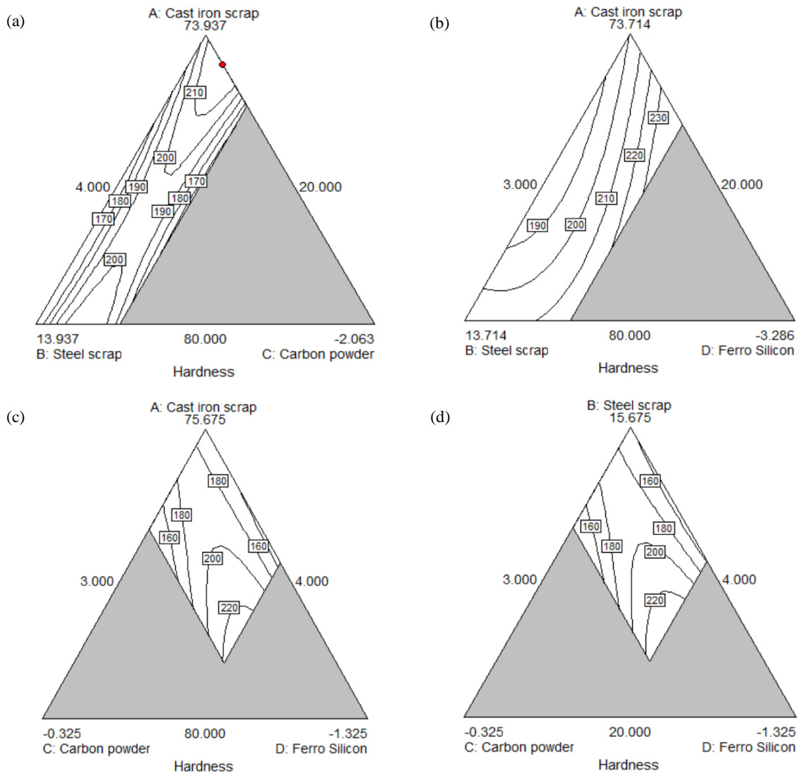
Fig. 3. Contour plots for hardness illustrated in various compositions
