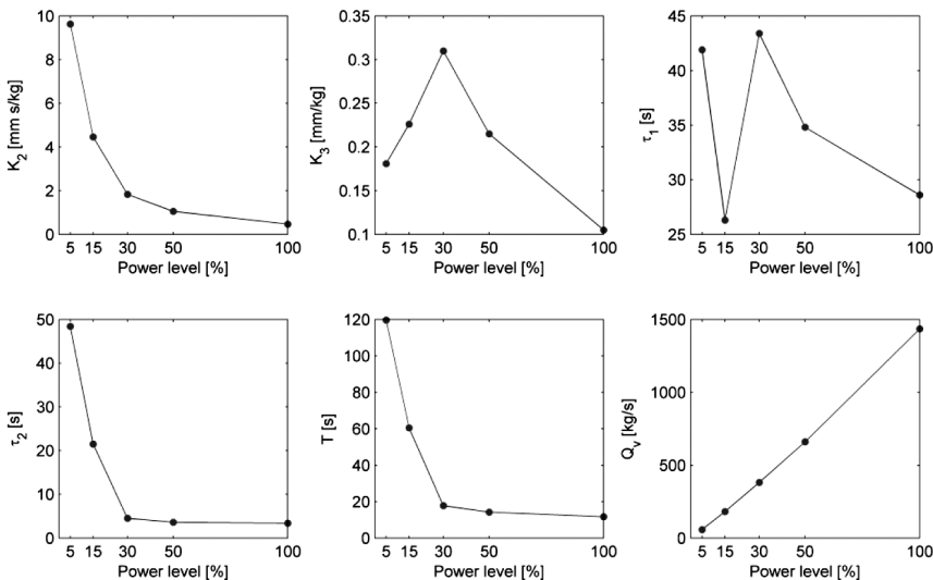
Fig. 2. Parameters of the steam generator model relative to thermal power transferred by primary side.
