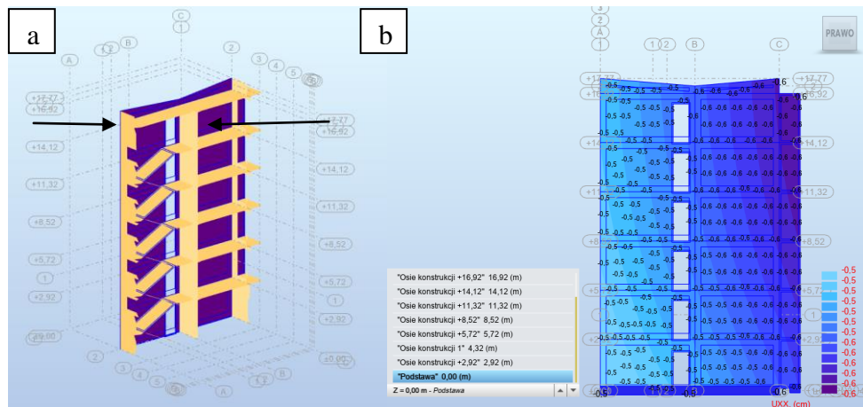
Fig. 5. Diaphragm stiffened by vertical communication structure: a) 3D diagram with an indication of the wall considered in the analysis; b) horizontal displacement u_x [cm] (Bieranowski P. 2019)
