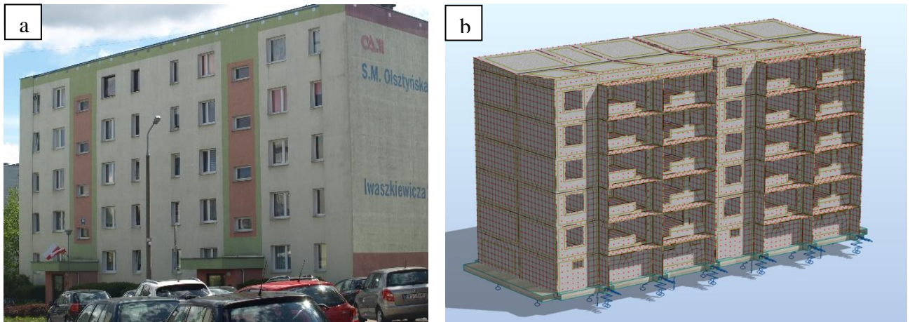
Fig. 1. Residential building of the Wk-70 large-panel system (F.D. Ilawa) - 5th floor: a) northern facade - photograph; b) southern facade - FEM 3D model of the building structure based on Winkler (Bieranowski P. 2018/19)
