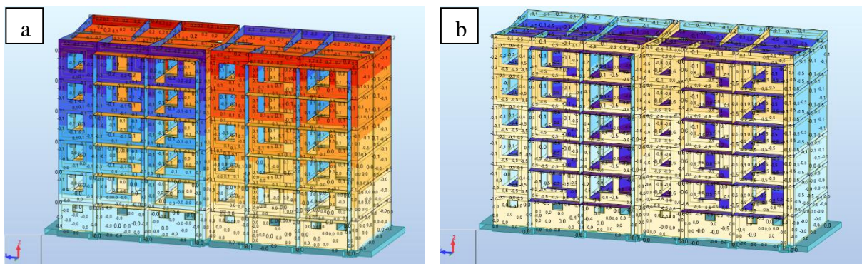
Fig. 4. Displacement values of the Wk-70 building structure: a) horizontal towards the global y axis; b) vertical towards the global z axis, horizontal displacement u_y [cm], vertical displacement w_z [cm], (Bieranowski. P. 2019)
