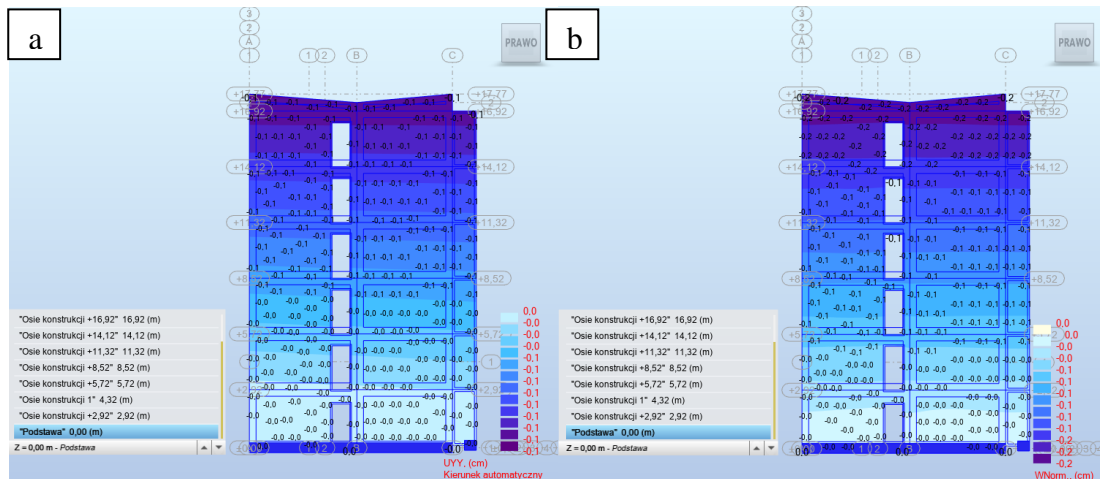
Fig. 6. Diaphragm stiffened by vertical communication structure: a) horizontal displacement u_y [cm]; b) vertical displacements w_z [cm] (Bieranowski P. 2019)
