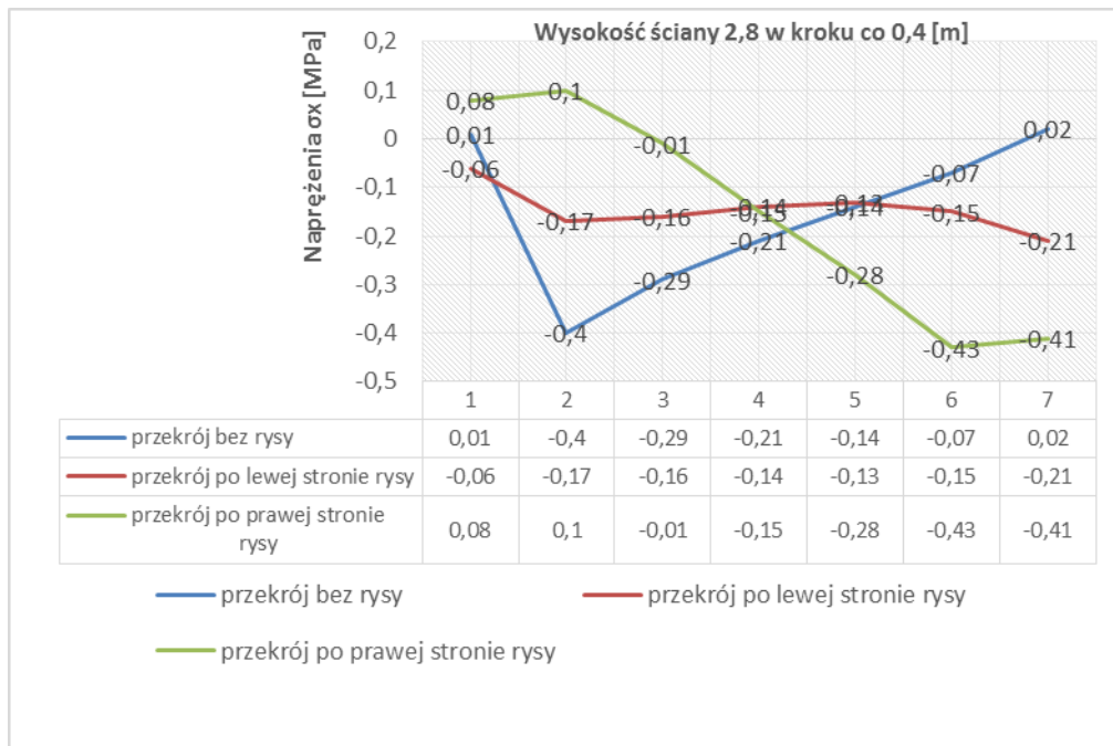
Fig. 8. Diagram of normal stresses in the direction of the local x axis for the cross section of a reinforced concrete panel wall, normal stress - \sigma_x [MPa], (Bieranowski P.2019)
