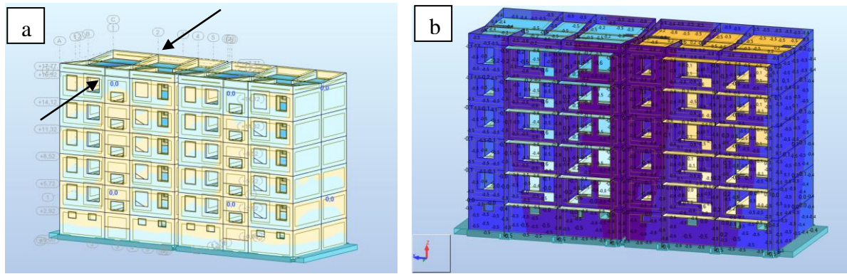
Fig. 3. The values of horizontal displacements towards the global x axis of the Wk-70 building structure: a) FEM model that does not take into account the cooperation of the building structure with the soil center; b) FEM model of the building structure in cooperation with the half-space of the soil center, horizontal displacement u_x [cm] (Bieranowski. P. 2019)
