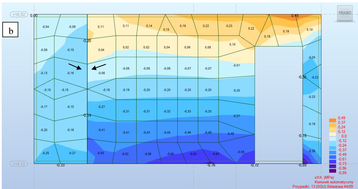
Fig. 7. FEM mesh with results for a separate part of the stiffening diaphragm - load-bearing wall of the last floor of the Wk-70 large-panel building: a) wall without scratching; b) a cracked wall, (Bieranowski P. 2019)
