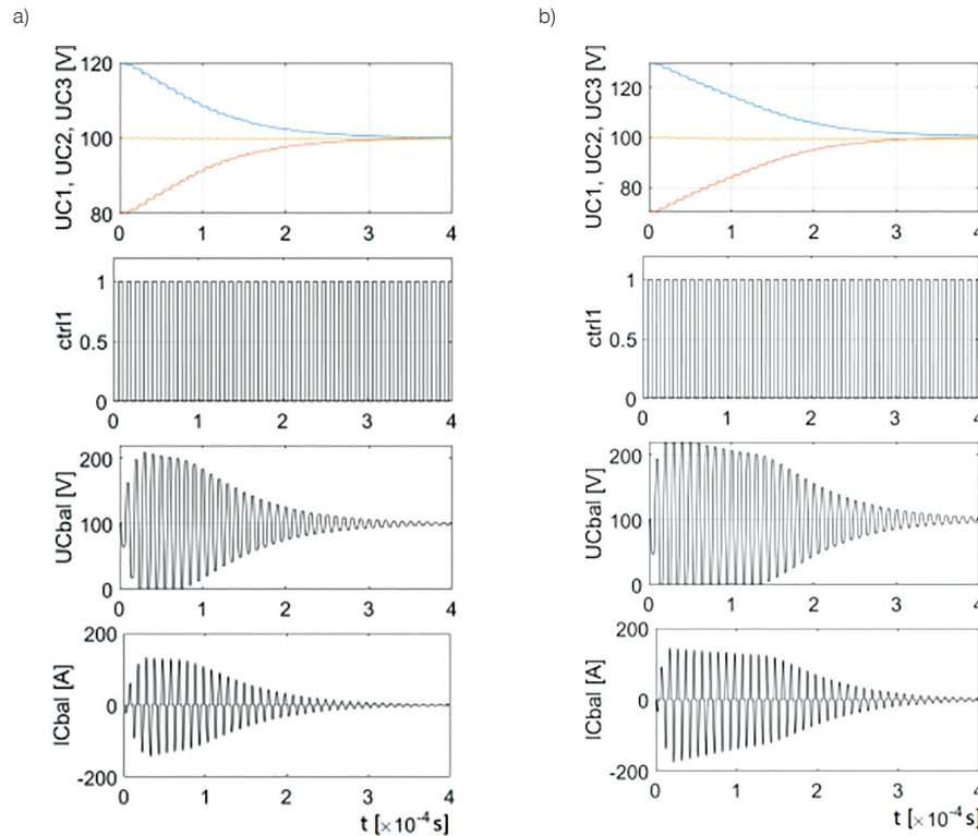
Fig. 8. The impact of initial voltages across series capacitors on the dynamics of the balancing process. Waveforms of voltages on series capacitors ( u_{C_1}, u_{C_2}, u_{C_3} ); the voltage and current on the balancing capacitor ( u_{Cbal}, i_{Cbal} ); control signal ( ctrl_1 ). Test cases: u_{C_1}(0) = 120\text{V}, u_{C_2}(0) = 80\text{V}, u_{C_3}(0) = 100\text{V} – energy transfer from C_1 to C_2 (a); u_{C_1}(0) = 130\text{V}, u_{C_2}(0) = 70\text{V}, u_{C_3}(0) = 100\text{V} – energy transfer from C_1 to C_2 (b). MATLAB/Simulink results
