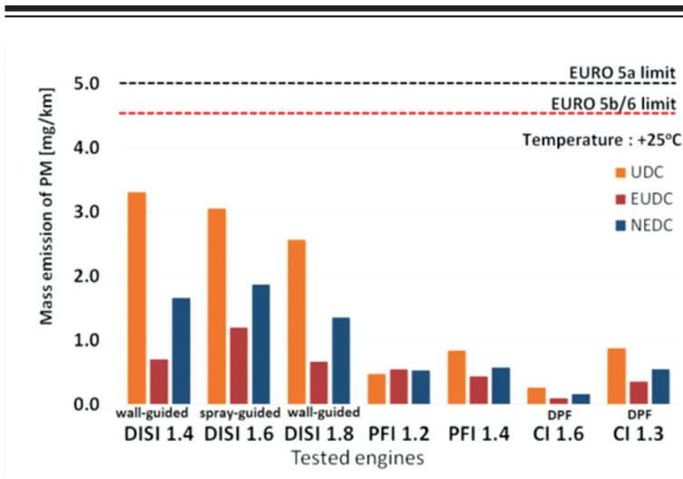
Fig. 5. Results of PM emission of various engines over the NEDC cycle [7]
