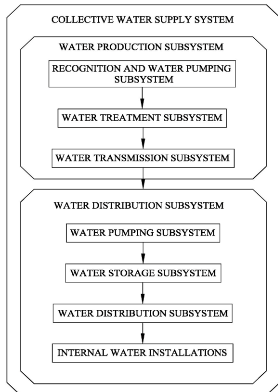
Figure 1. Block diagram of the collective water supply system
