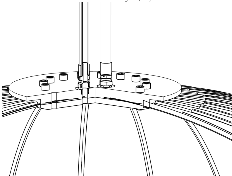
Figure 12 Visualization of a conceptual compressed air tank that could be used for offshore wind turbines (compiled on the basis of 18, 19)
