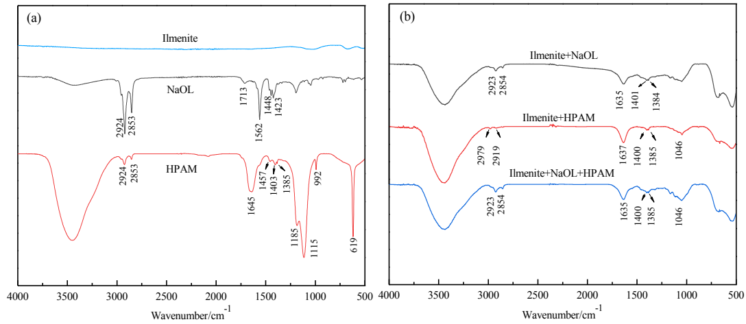
Fig. 6. Infrared spectra of ilmenite under different pharmaceutical systems
