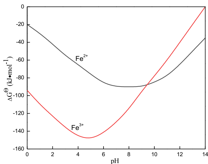
Fig. 8. Standard Gibbs free energy ( \Delta G^0 ) for metal ions reacting with sodiumoleate as a function of the pH value
