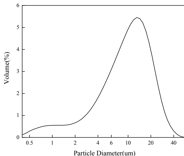
Fig. 2. Particle size analysis of raw ore
