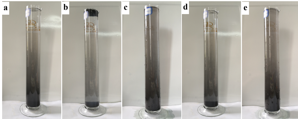
Fig. 3. Flocculation image of fine ilmenite. Left to right picture shows (a) blank group, (b) with sodium oleate, (c) with soluble starch, (d) with polyacrylamide, (e) with sodium carboxymethyl cellulose
