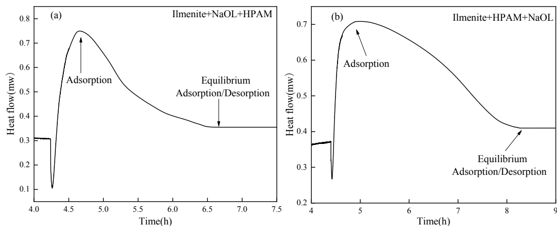
Fig. 7. Typical microcalorimetric curve for adsorption on ilmenite surface
