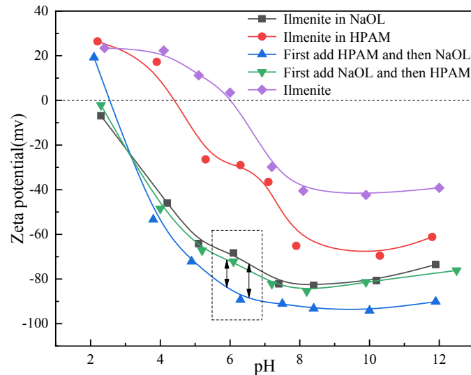
Fig. 5. Relationship between Zeta potential and pH of ilmenite after flocculant action
