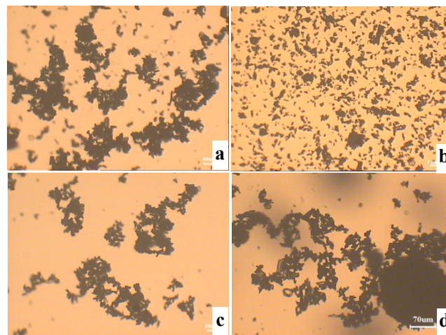
Fig. 4. Micrograph analysis results. Figures a, b, c and d represent respectively addition of 2 \times 10^{-4} mol/L sodium oleate group, 80 g/t polyacrylamide group, 2 \times 10^{-4} mol/L sodium oleate first and then 80g/t polyacrylamide group, first 80g/t polyacrylamide and then 2 \times 10^{-4} mol/L sodium oleate group
