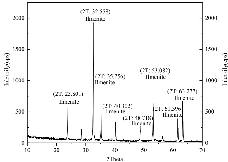
Fig. 1. X-ray diffraction (XRD) spectrum of the purified ilmenite sample
