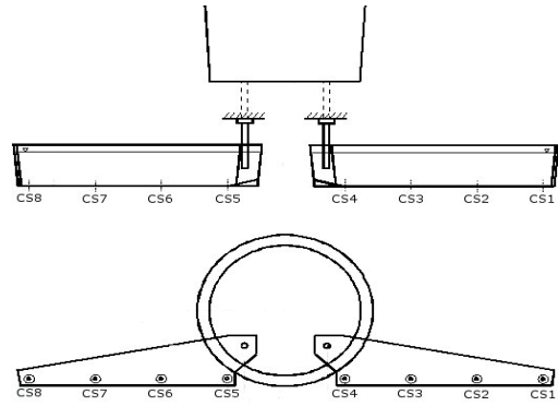
Fig. 1 Configuration of the ladle and tundishes in CCM2
