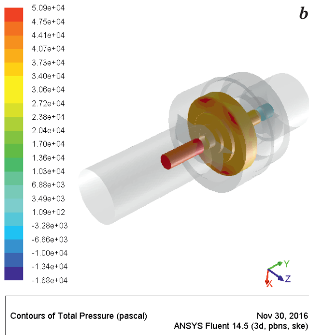
Fig. 6. Distribution of total pressure on the head of the impulse valve in variant 1 (a) and variant 2 (b)
