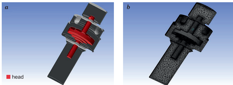
Fig. 5. Area of water flow inside the impulse valve: geometry (a) and the numerical grid (b)
