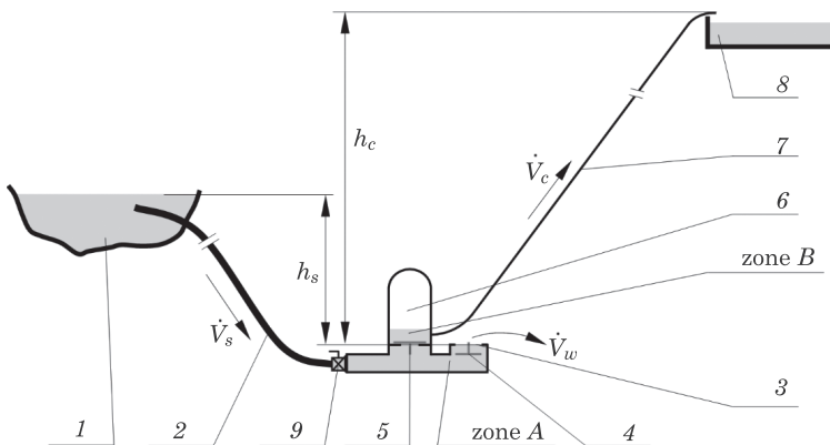
Fig. 1. Diagram of a water ram: 1 – water source, 2 – drive pipe, 3 – impulse valve, 4 – closing element of the impulse valve, 5 – pressure valve, 6 – air chamber, 7 – delivery pipe, 8 – water collector, 9 – shut-off valve, h_s – height of the water supply source, h_c – height of water outflow (delivery head), \dot{V}_s – flow rate of water supply, \dot{V}_c – rate of water outflow to the water collector, \dot{V}_w – rate of water outflow to the surrounding environment; zone A – working zone, zone B – pressure zone; the impulse valve and the check valve are one-way (non-return) valves
