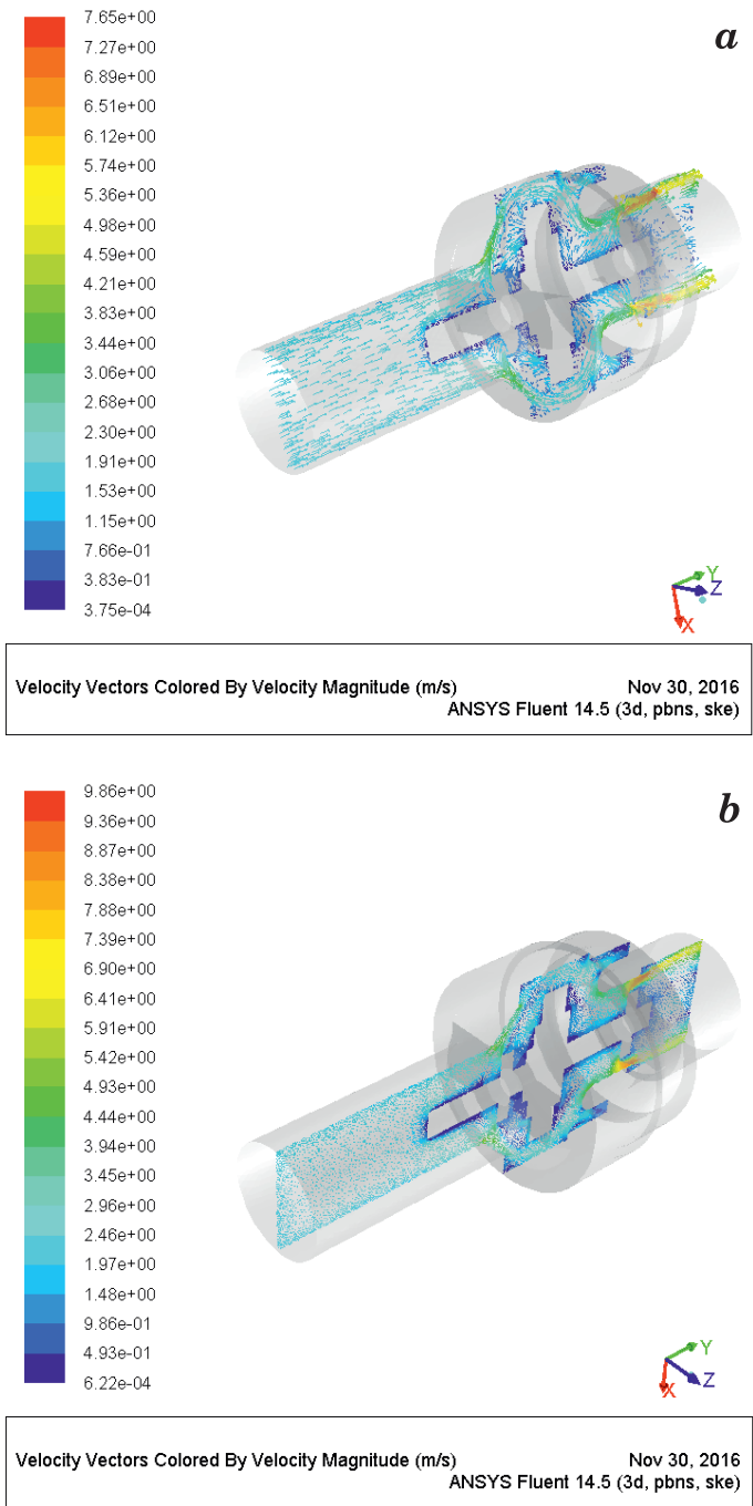
Fig. 7. Velocity fields for selected longitudinal cross-sections of the impulse valve in variant 1 (a) and variant 2 (b)
