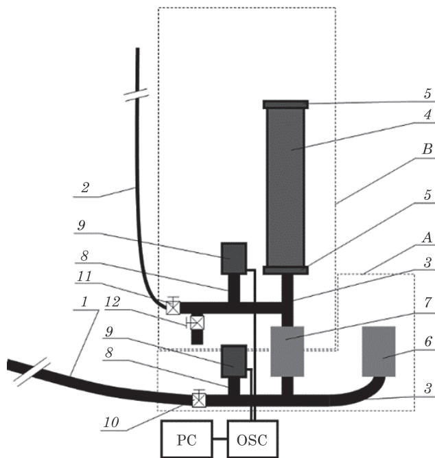
Fig. 2. Diagram of the experimental installation
