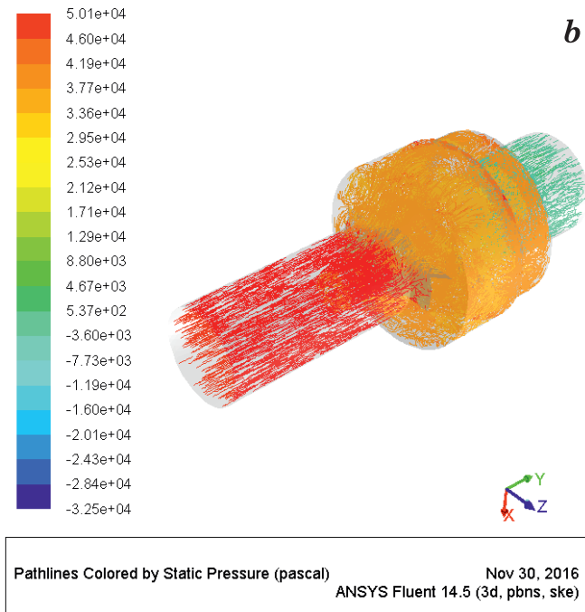
Fig. 8. Path lines colored according to pressure in variant 1 (a) and variant 2 (b)
