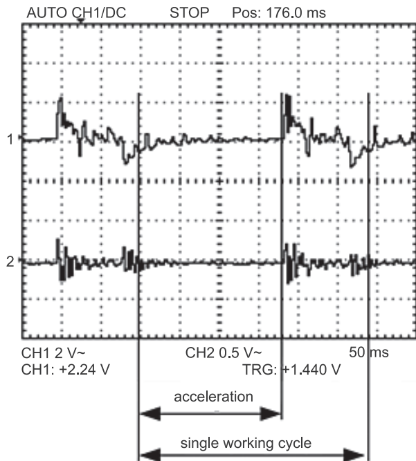
Fig. 3. Changes in pressure during a single working cycle of a water ram
