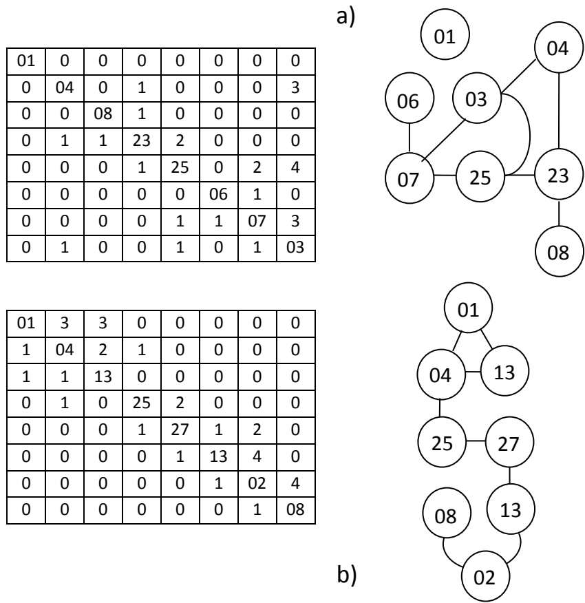
Fig. 5. Interim results of packing machine structure optimization synthesis using GA [source: own study]
