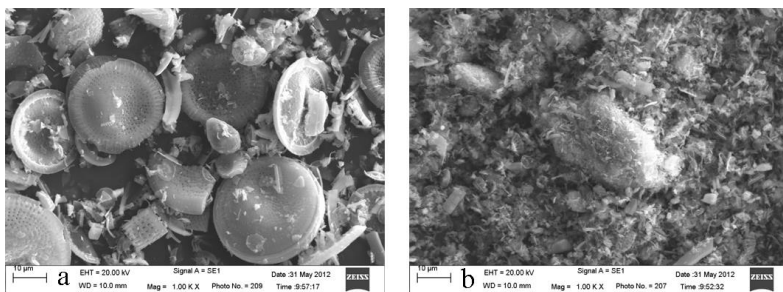
Fig. 7. SEM comparison of the diatomite purification (a: concentrate, b: tailings)
