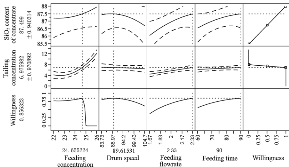
Fig. 6. Prediction profiler for optimal configuration
