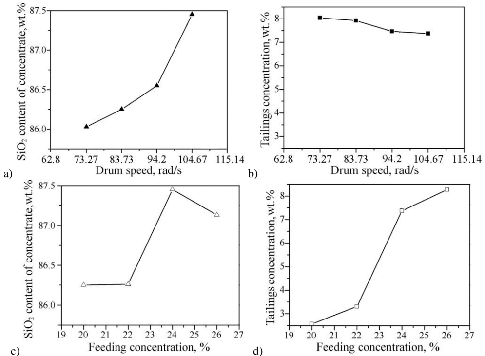
Fig. 4. Influence of drum speed and feeding concentration on laminar-flow centrifugal separation
