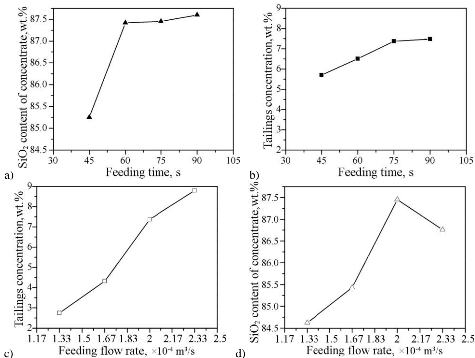
Fig. 5. Influence of feeding time and feeding flow rate on laminar-flow centrifugal separation
