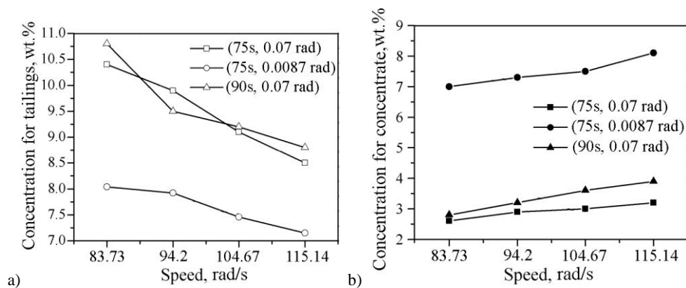
Fig. 3. Influence of cone angle and drum speed on laminar-flow centrifugal separation
