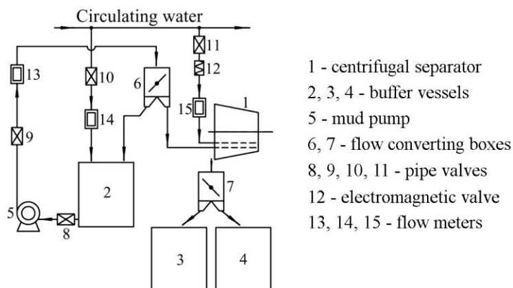
Fig. 2. Pilot-scale experiment flow sheet
