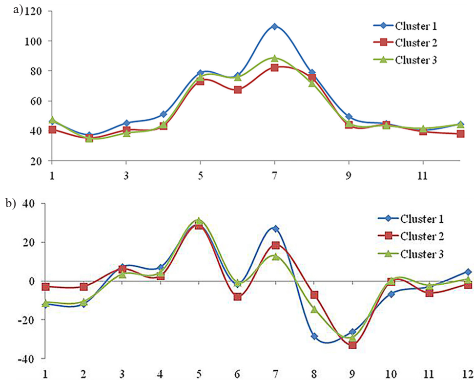
Figure 7. Annual precipitation trend by months within clusters (Abscissa – order of months in year; (a) clusters distinguished on the basis of Euclidean distance, axis of ordinate – precipitation, mm; (b) clusters distinguished on the basis of Pearson's distance; axis of ordinate – derivative of precipitation (growth in comparison with the previous month), mm/month)
