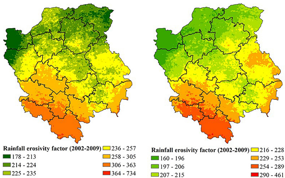
Figure 9. Spatial variation of rainfall erosivity factor ( \text{MJ mm ha}^{-1} \text{h}^{-1} per year)
