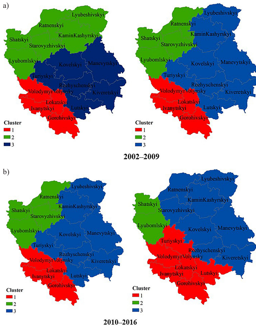
Figure 8. Cluster analysis of precipitation trend by districts within a year (a) Euclidean distance, (b) Pearson's distance
