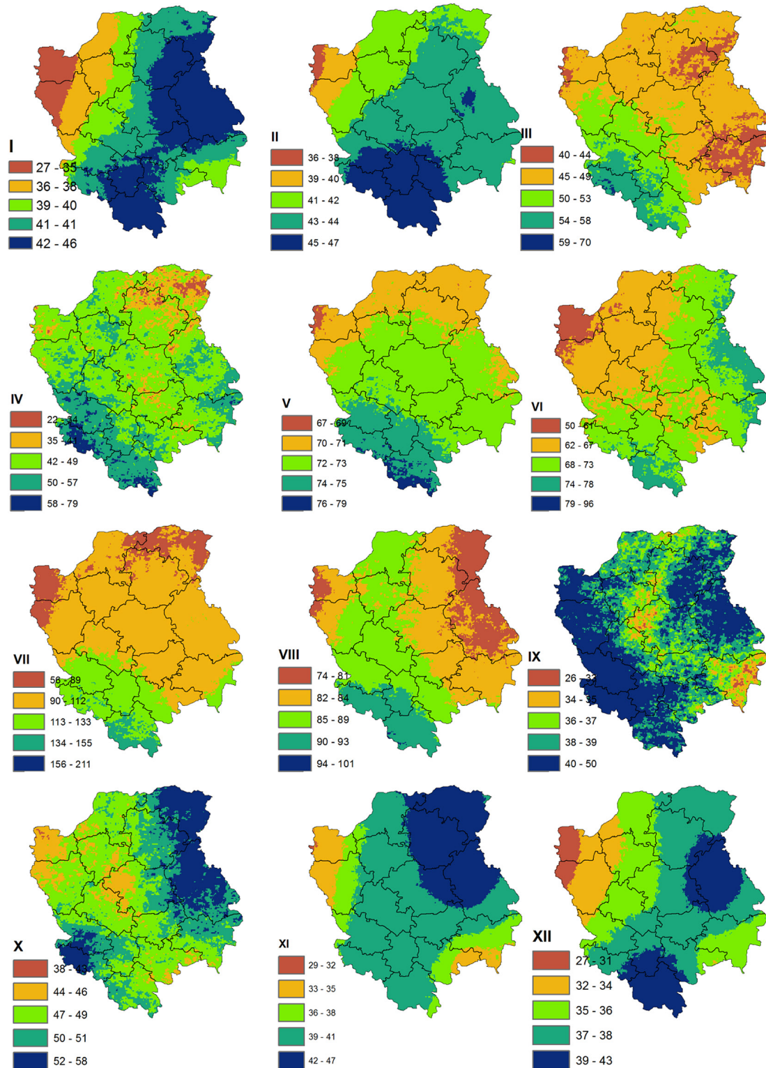
Figure 4. Spatial variation of monthly precipitation in 2002–2009 (I – January, II – February, III – March, IV – April, V – May, VI – June, VII – July, VIII – August, IX – September, X – October, XI – November, XII – December)
