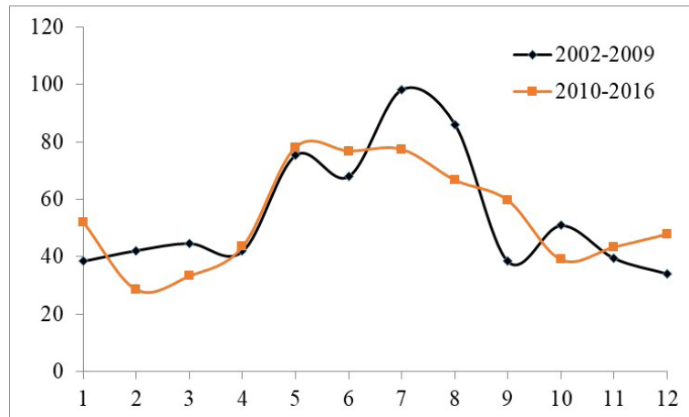
Figure 2. Monthly dynamics of precipitation in (a) 2002–2009 and (b) 2010–2016. Abscissa – order of months of the year, axis of ordinates – precipitations, mm
