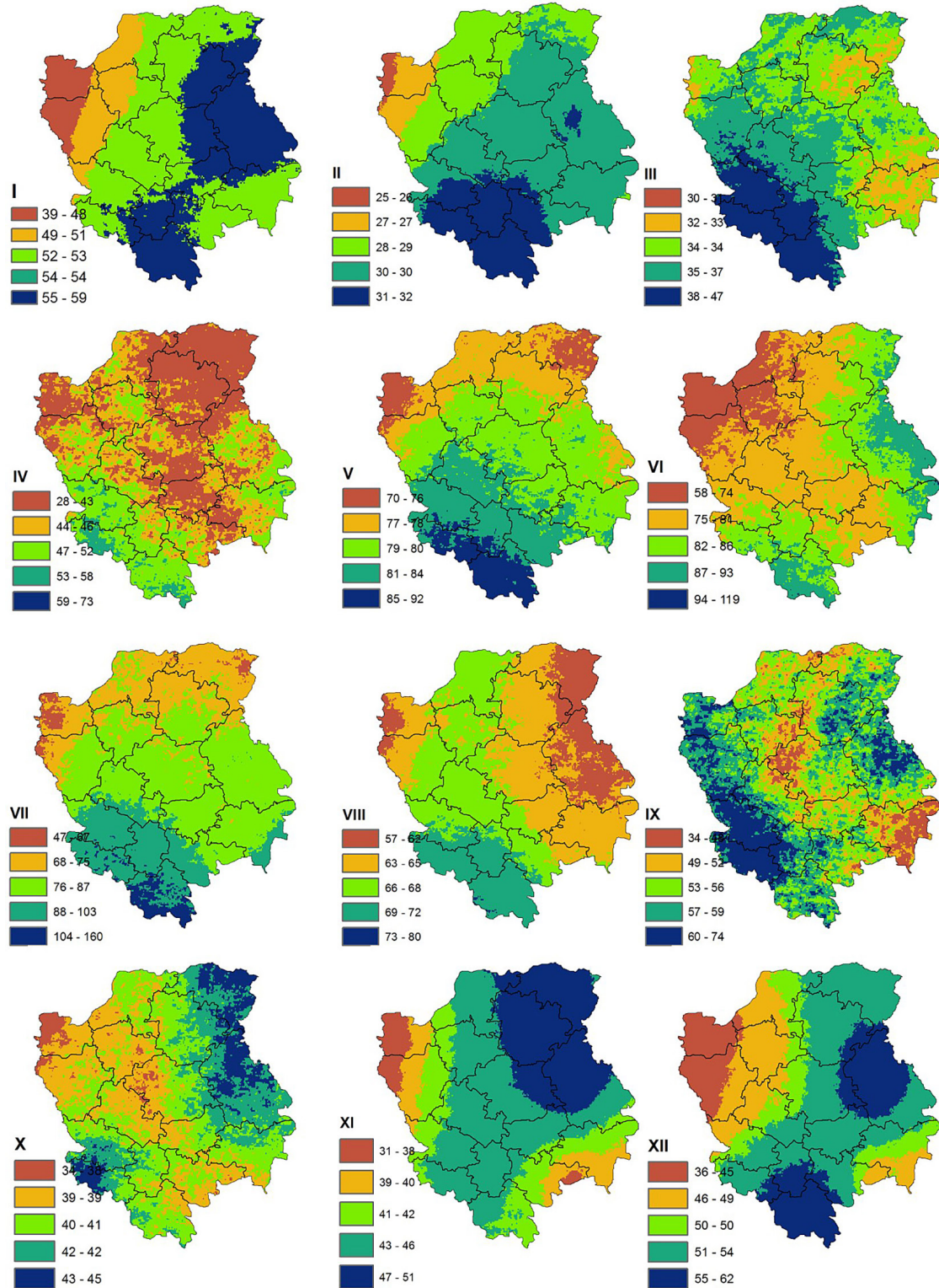
Figure 5. Spatial variation of monthly precipitation in 2010–2016 (I – January, II – February, III – March, IV – April, V – May, VI – June, VII – July, VIII – August, IX – September, X – October, XI – November, XII – December)
