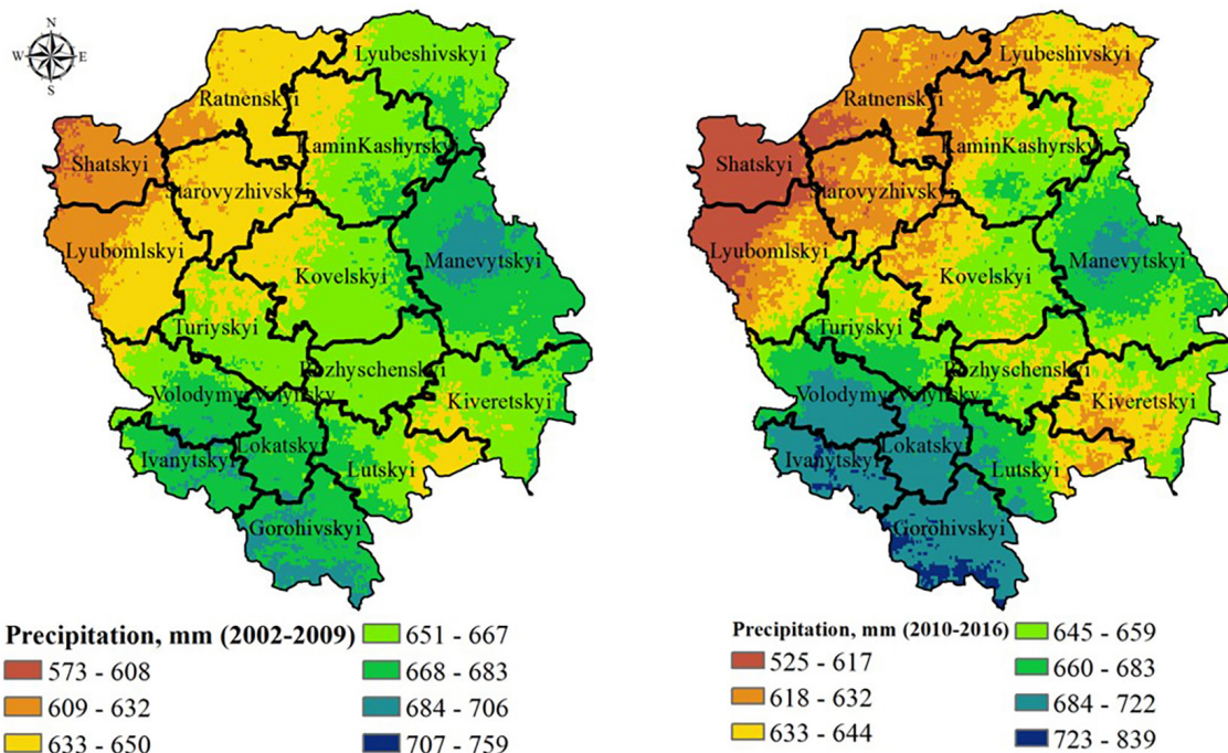
Figure 3. Spatial distribution of annual precipitation
