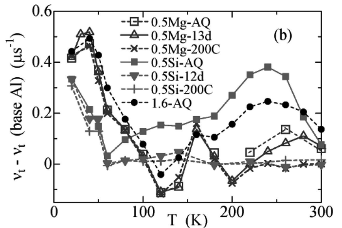
Fig. 3(b) Temperature variations of trapping rates caused by solute Mg or Si atoms for Al-0.5%Mg or Al-0.5%Si sample
