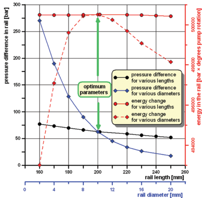
Fig. 9. Calculated pressure differences and energy changes for various rail dimensions
