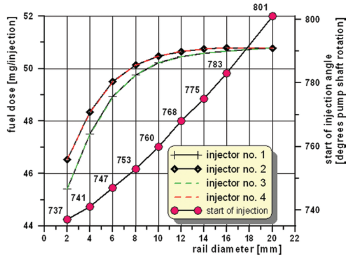
Fig. 8. Calculated dose and angle of start of injection values for various rail diameters
