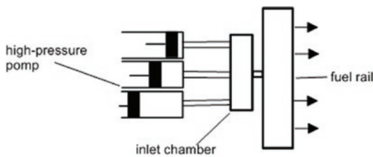
Fig. 1. Schematic of the modelled fuel supply system
