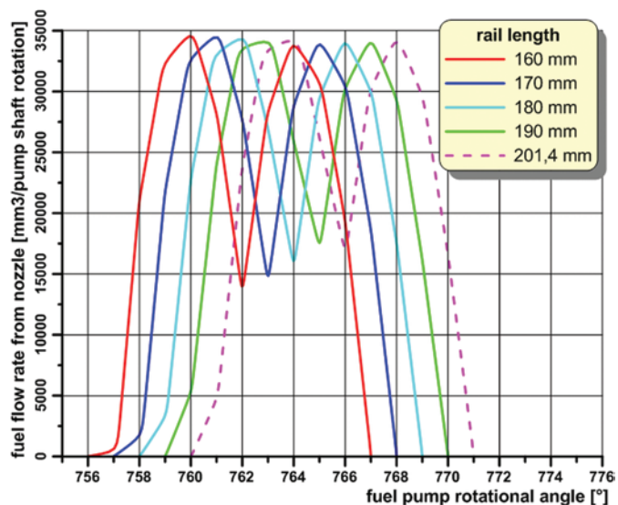
Fig. 2. Calculated injection traces for rail lengths 160 mm – 201.4 mm
