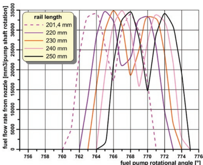
Fig. 3. Calculated injection traces for rail lengths 201.4 mm – 250 mm
