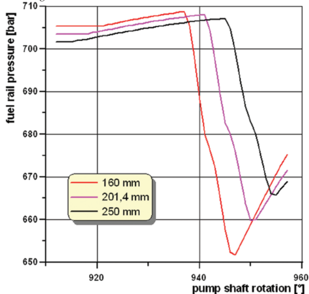
Fig. 5. Calculated pressure changes in the rail during the injection event, together with angles of start of injection for selected rail lengths
