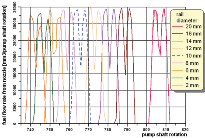
Fig. 6. Calculated injection traces for various rail diameters
