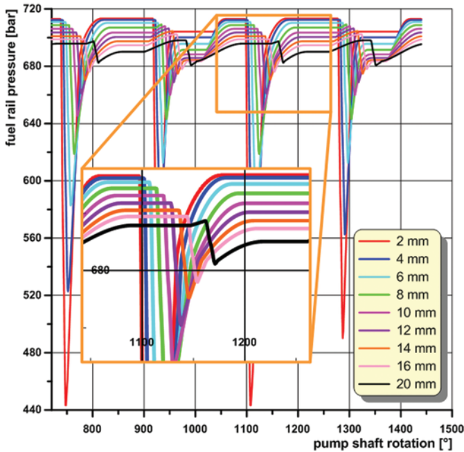
Fig. 7. Calculated pressure traces for various rail diameters
