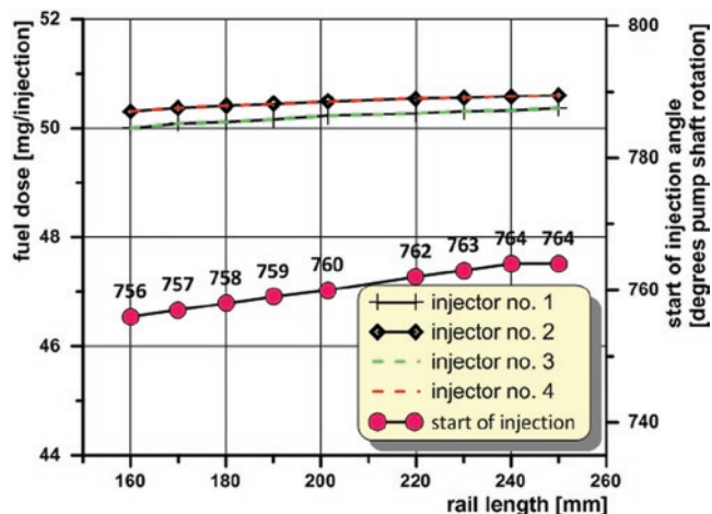
Fig. 4. Calculated fuel doses and angles of start of injection for various rail lengths
