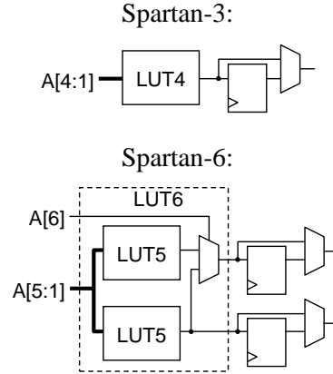
Figure 1. Simplified structure of the logic cell in Spartan-3 and Spartan-6 architectures
