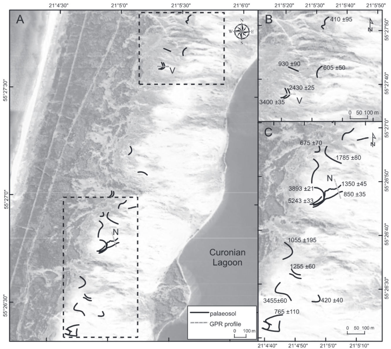
Fig. 2. Distributions of exposed palaeosols along the western slope of the Great Dune Ridge – a brighter shade on the photo-image indicates areas free of vegetation
