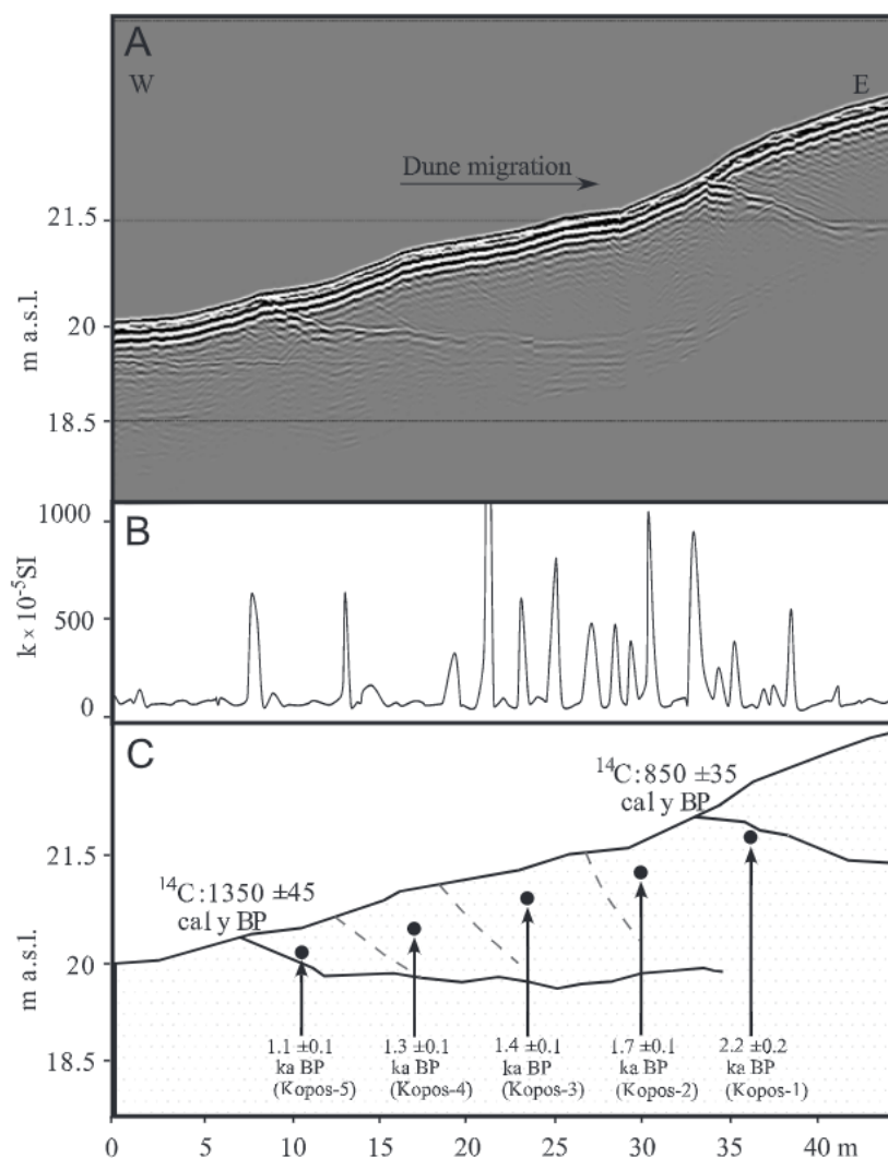
Fig. 5. Profile of detailed investigations at the Naglis dune site
