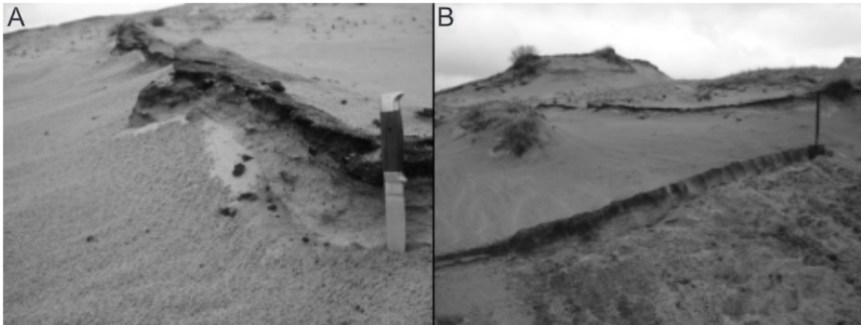
Fig. 3. Segments of exposed palaeosols on the Great Dune Ridge western slope in the vicinity of the Naglis dune site on the Dead (Grey) Dune ridge: a single palaeosol exposed by deflation (A); in many places, palaeosols of different age are situated near each other (B)
