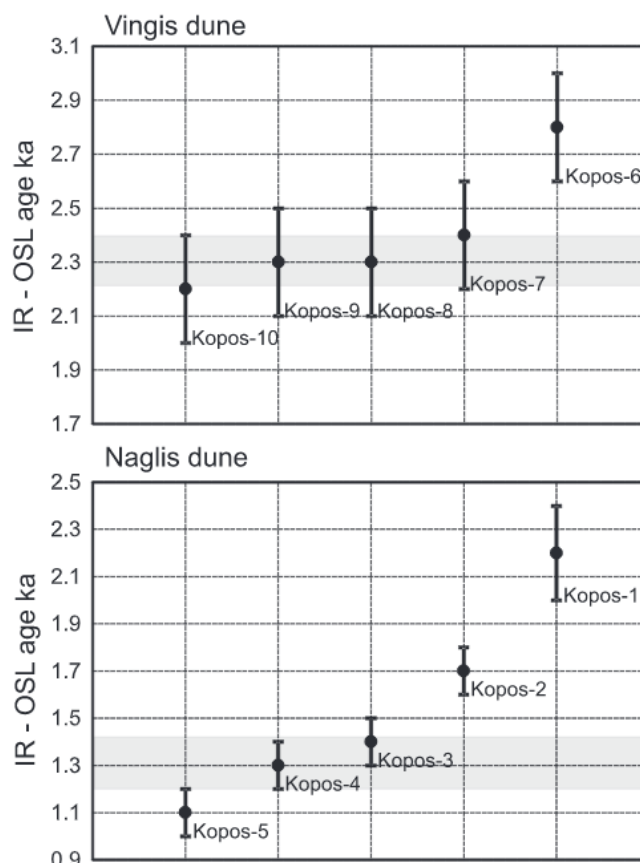
Fig. 7. Results of IR-OSL dating from the Vingis and Naglis dune sites
