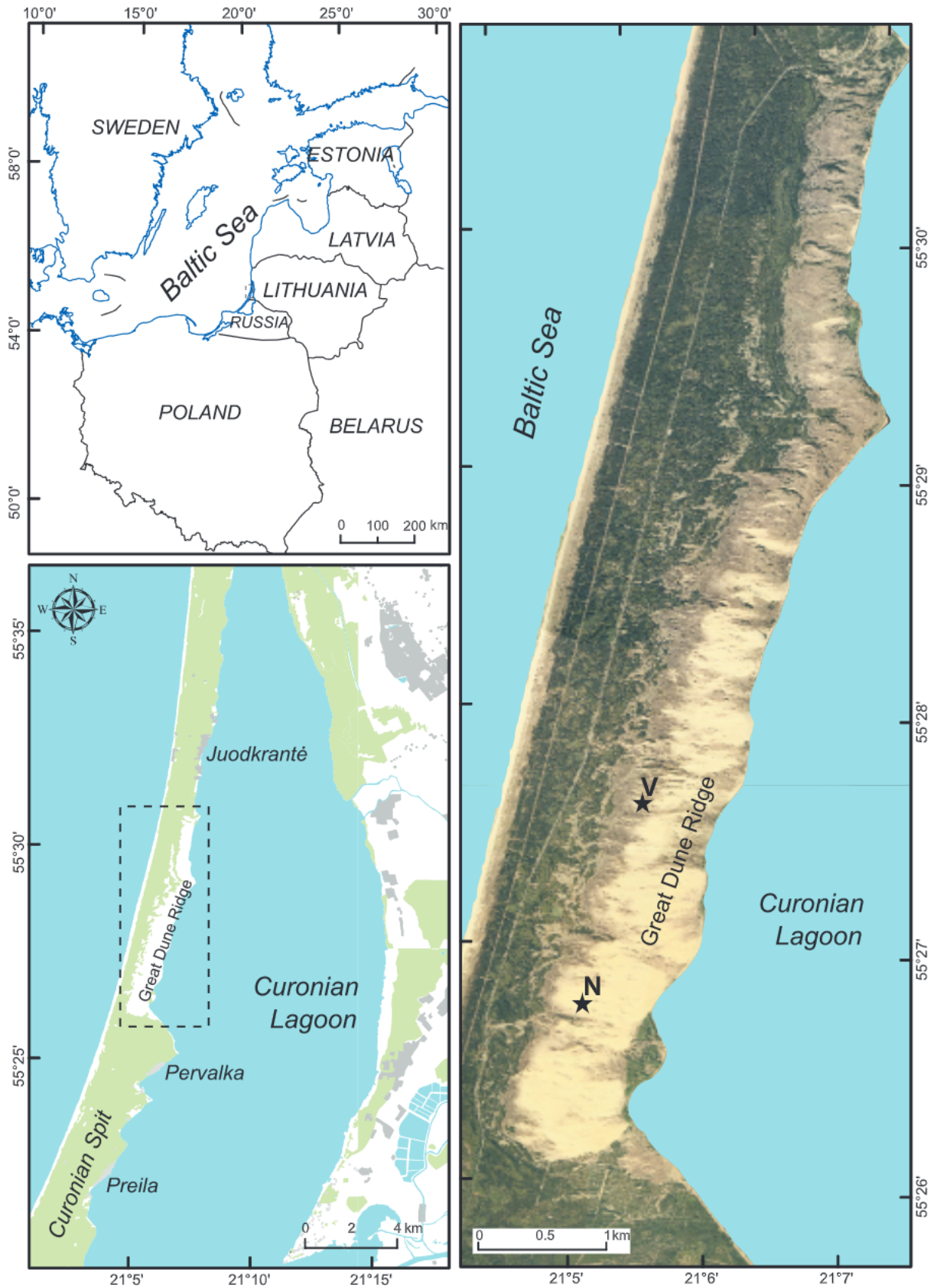
Fig. 1. Study area on the Curonian Spit
