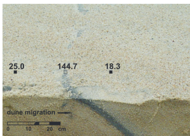
Fig. 6. Section of aeolian sediments along the GPR profile at the Naglis dune site
