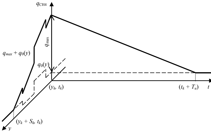
Fig. 1. Spatio-temporal relationship of methane release rate from the longwall cut with a shearer. Designation: y_k – location of the shearer at the longwall at time t_k ; S_k – length of the fracture zone in front of the shearer; T_u – methane emission stabilisation time after opening new face surface; q_0(y) – distribution of the initial value of the methane volume flow per area unit of the longwall, taking into account the variable gas distribution of the seam; q_{\max} – increase of methane density of the volume stream at the mining site
