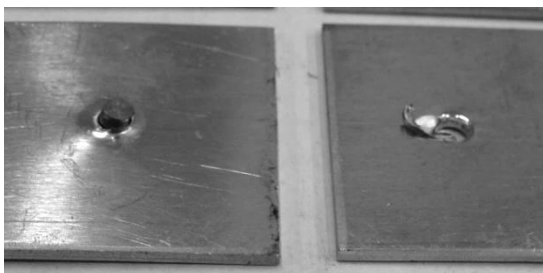
Fig. 5. SSPR joints of the aluminium alloys sheets after the laps separation
