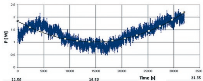
Fig. 23. Distribution of power delivered by the wind turbine on 29 October 2014
