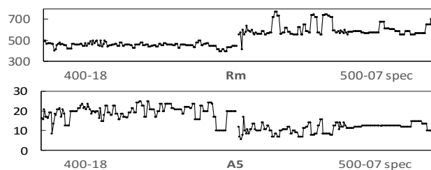
Fig. 1. Examples of typical run charts for the two process output variables (ductile iron ultimate tensile strength Rm and elongation A5) extracted from the data sets No 1, 3 and 5
