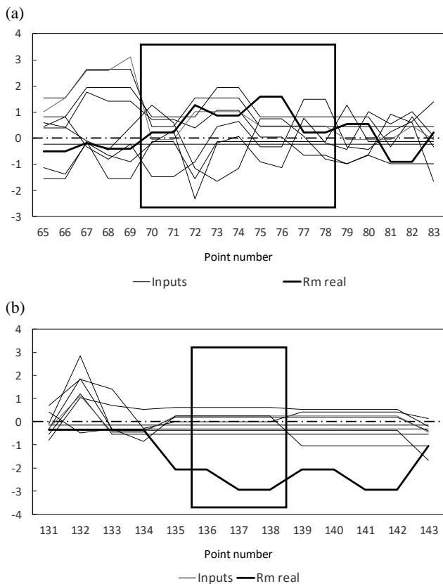
Fig. 8. Examples of run charts with abnormal patterns of the process output only and with absence of noticeable correlations: (a) dataset no. 2, pattern type 2; (b) dataset no. 1, pattern type 5
