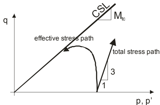
Fig. 2. Stress path in conventional triaxial compression
