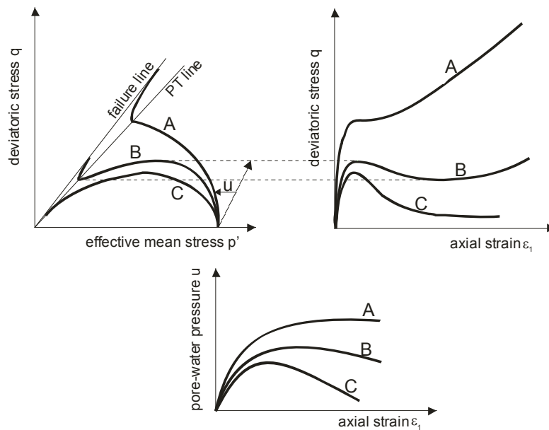
Fig. 3. Static liquefaction
