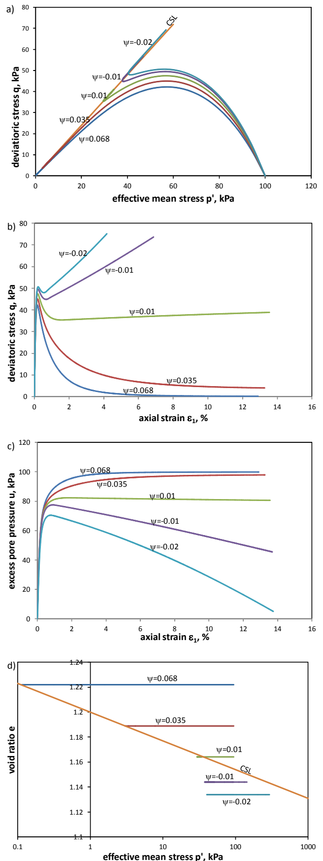
Fig. 8. Results of numerical simulations of undrained triaxial compression
