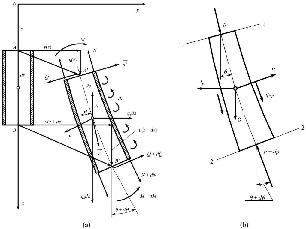
Fig. 1. Diagram of forces and moments acting on pipe element (a) and fluid element in pipe (b)
